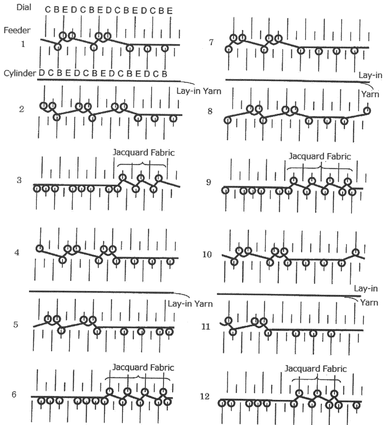
FIG. 6B COMPARATICE EXAMPLE 2: JACQUARD FABRIC
