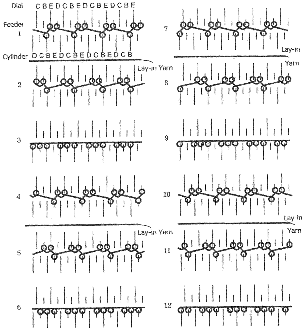
FIG. 6A COMPARATIVE EXAMPLE 2: BACKGROUND STRUCTURE
