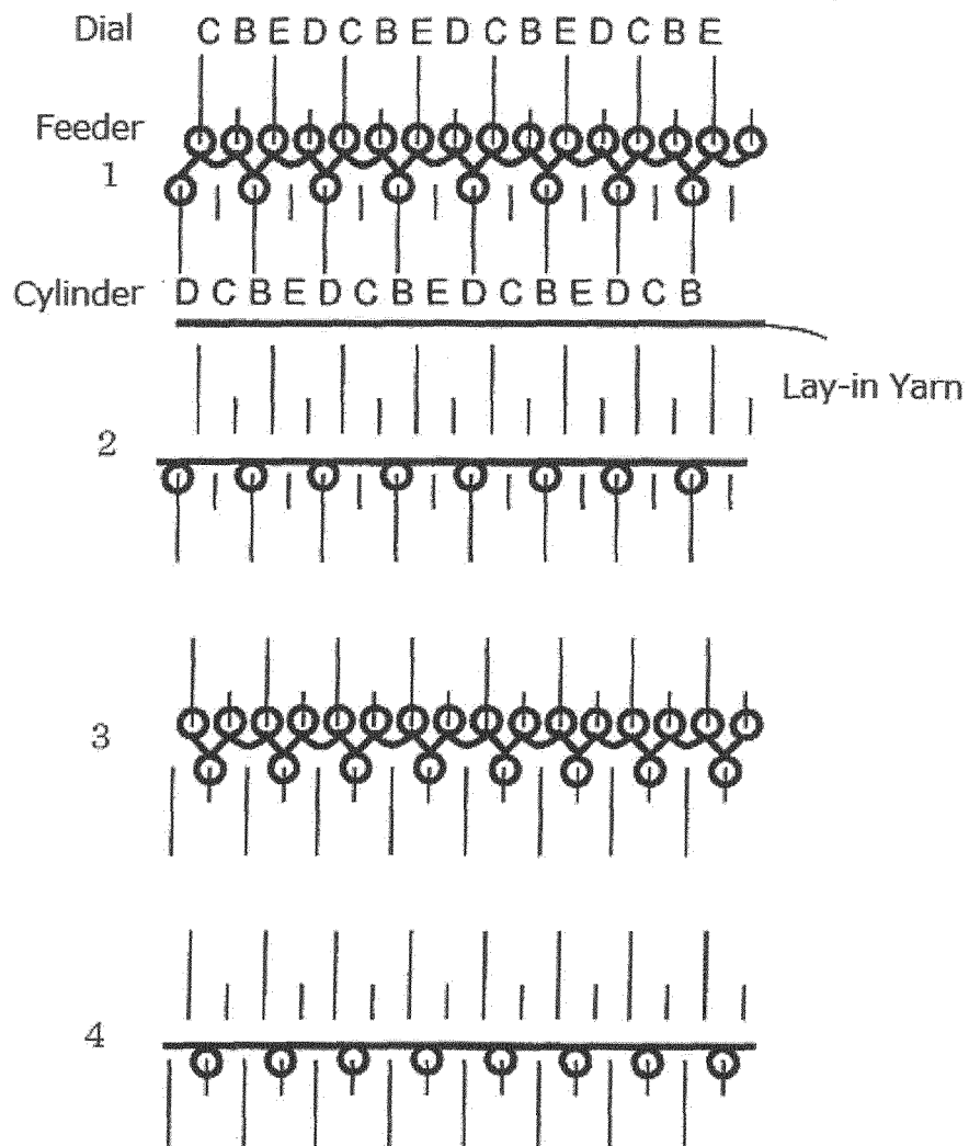
FIG. 4A COMPARATIVE EXAMPLE 1: BACKGROUND STRUCTURE
