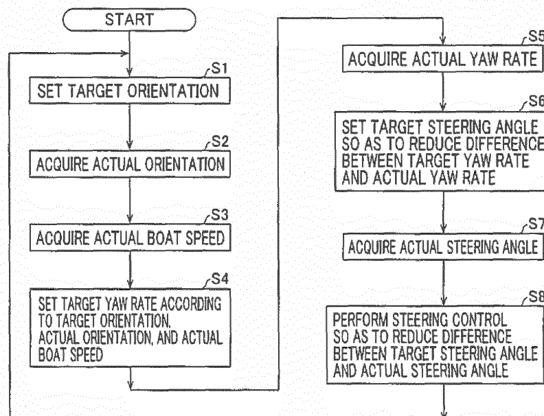
FIG.11 ORIENTATION CONTROL PROCESSING
