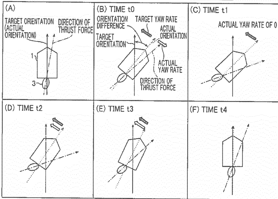
FIG.6 EXAMPLE OF OPERATION OF ORIENTATION CONTROL
