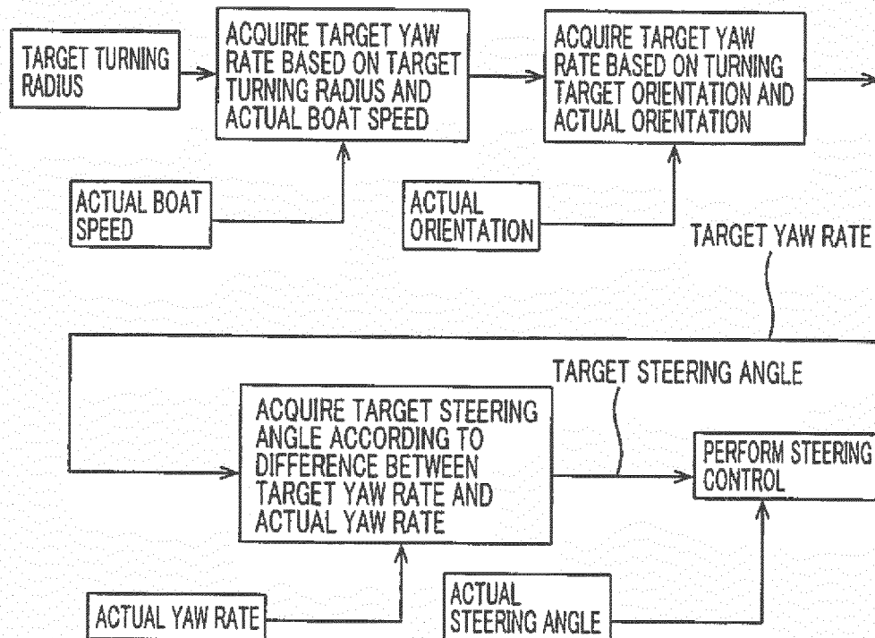
FIG.7 CONTROL LOGIC FOR TURNING CONTROL
