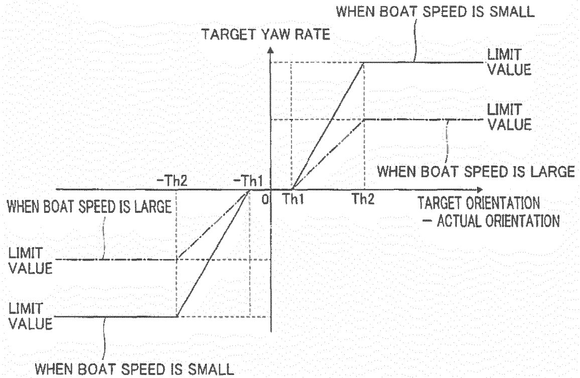
FIG.4 RELATIONSHIP BETWEEN DIFFERENCE BETWEEN TARGET ORIENTATION AND ACTUAL ORIENTATION AND TARGET YAW RATE (DURING ORIENTATION CONTROL)
