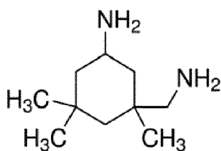
Isophorone diamine; and a mixture thereof.
