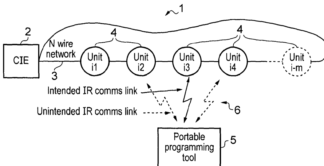
System level overview block diagram
