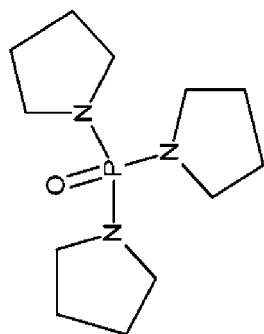
Tris(dimethylamino)phosphine
