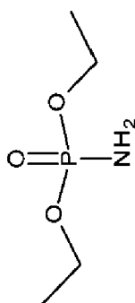
Diethyl phosphoramidate
