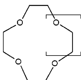
Crown ethers 1-3
