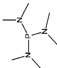
Tris(dimethylamino)phosphine
