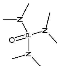
Hexamethylphosphoramide
