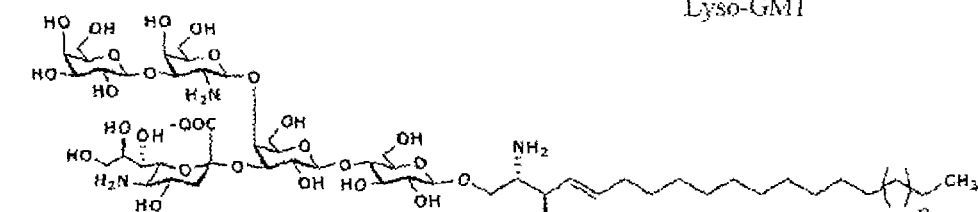
Deacetyl-lyso-GM1
