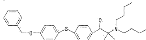
Compound No. 28
