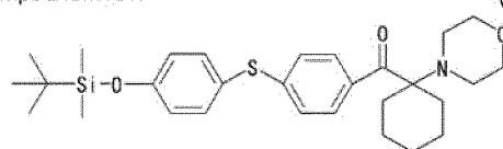
Compound No. 21
