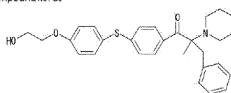
Compound No. 27
