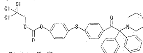
Compound No. 26
