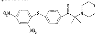
Compound No. 26
