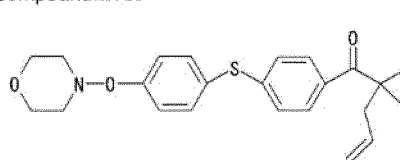
Compound No. 25
