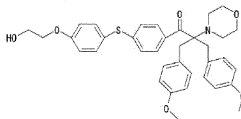
Compound No. 31
