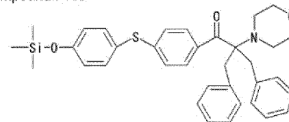
Compound No. 24
