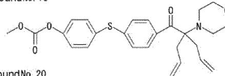
Compound No. 20
