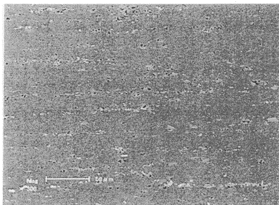
Fig. 2B Extruded material
