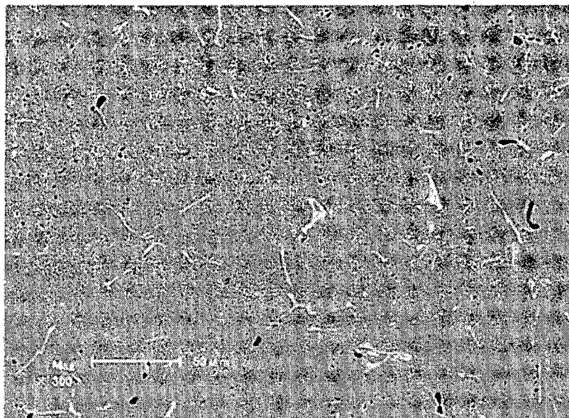
Fig. 3A Billet after homogenization treatment
