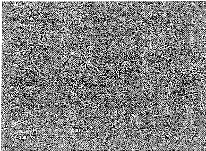
Fig. 2A Billet after homogenization treatment
