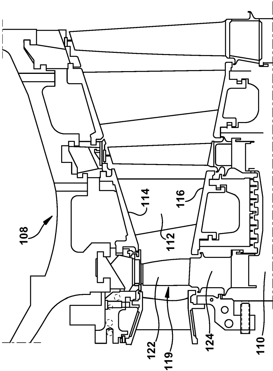
Fig. 2 (Prior Art)
