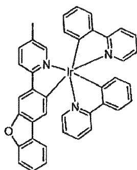
Compound 56
