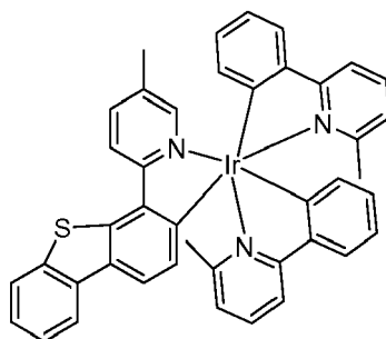
Compound 82
