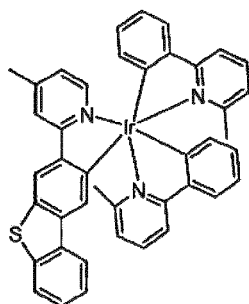
Compound 23
