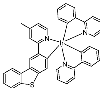
Compound 21
