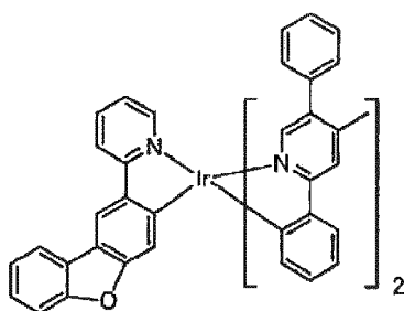
Compound 39
