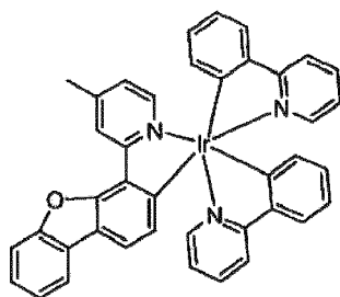
Compound 7
