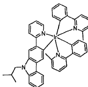
Compound 29
