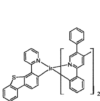
Compound 61
