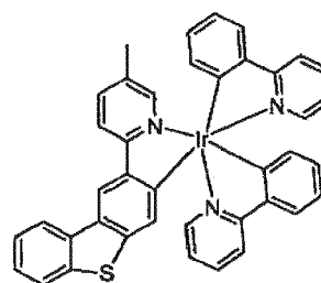
Compound 81
