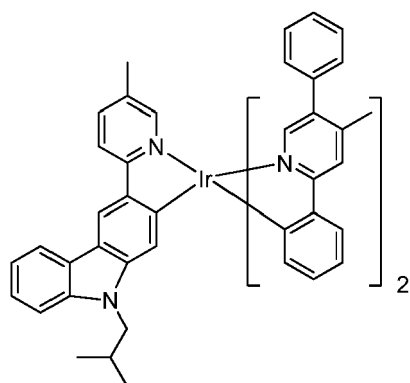
Compound 93
