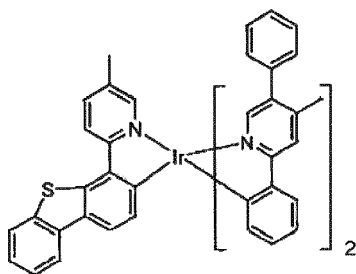
Compound 67
