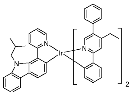
Compound 94
