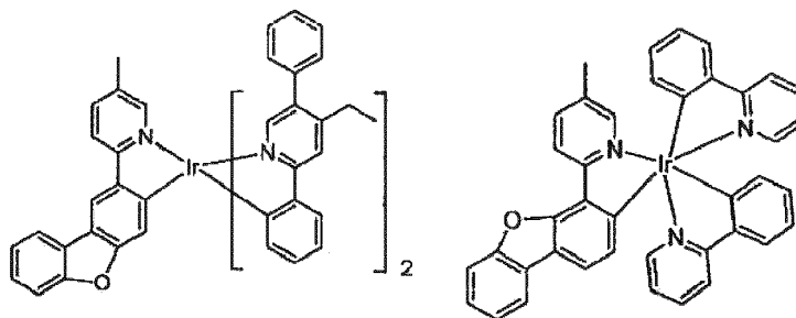
Compound 54
