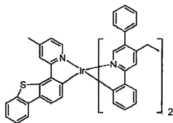
Compound 73
