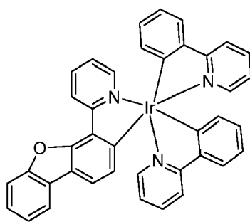
Compound 1
