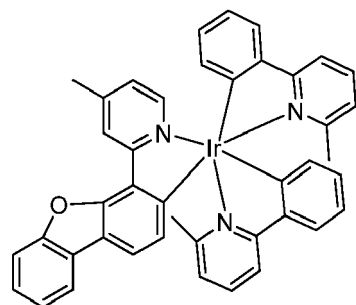
Compound 10
