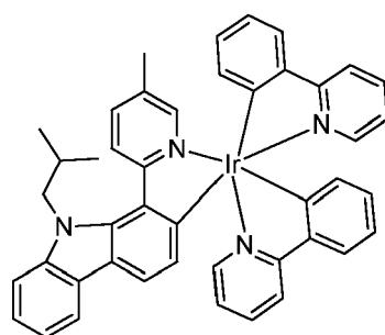
Compound 103
