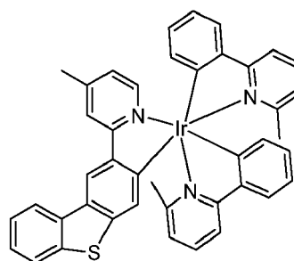
Compound 24
