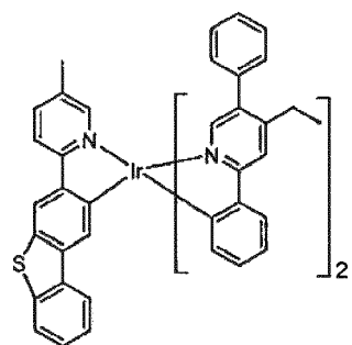
Compound 77
