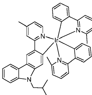
Compound 36
