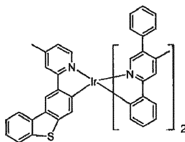
Compound 66
