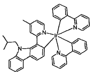
Compound 31
