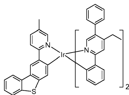
Compound 75
