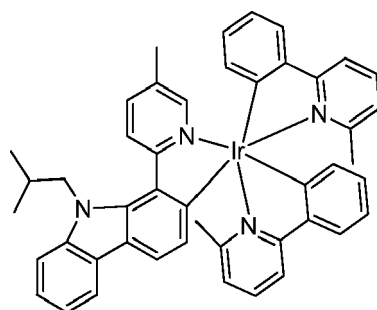
Compound 106
