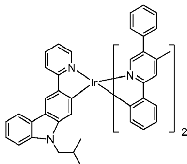
Compound 87
