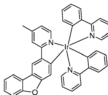
Compound 9
