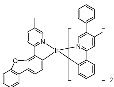
Compound 43
