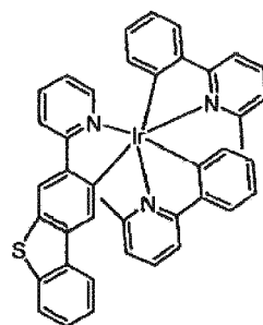
Compound 17
