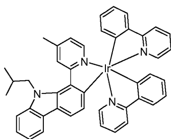
Compound 31
