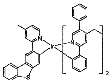
Compound 75
