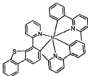
Compound 16
