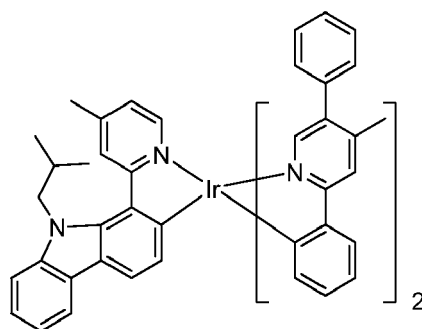
Compound 88
