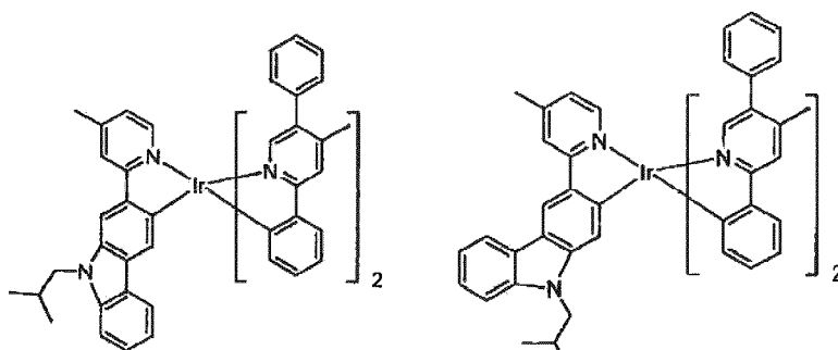
Compound 89
