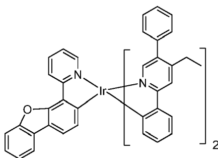
Compound 46
