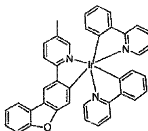
Compound 57
