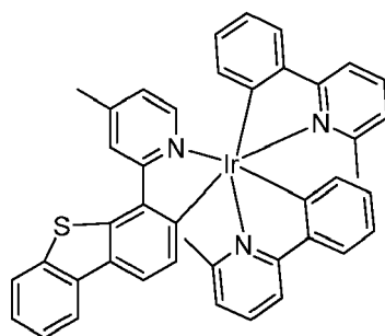
Compound 22
