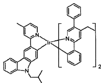
Compound 99
