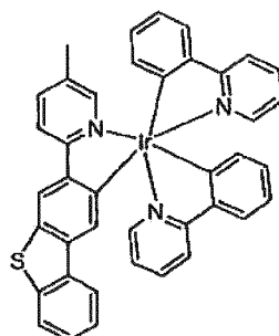
Compound 80
