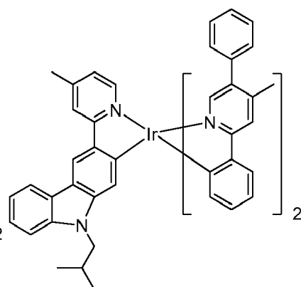
Compound 90
