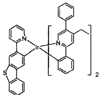
Compound 71
