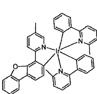
Compound 58
