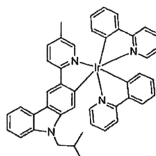
Compound 105
