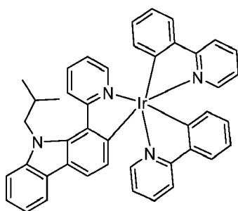
Compound 25
