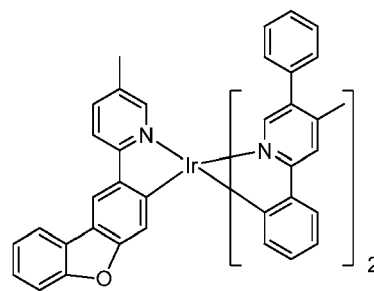
Compound 45
