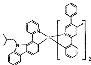
Compound 85
