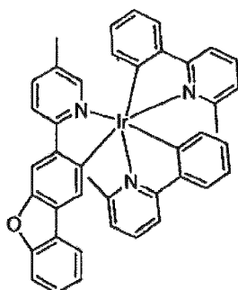
Compound 59
