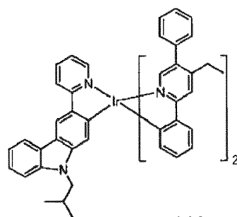
Compound 96
