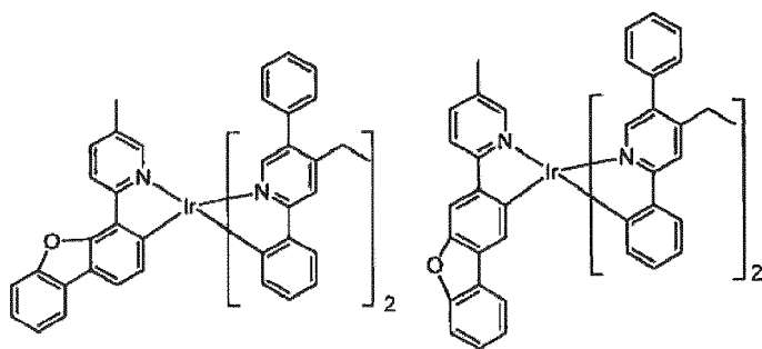
Compound 52
