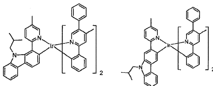
Compound 91
