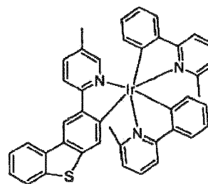
Compound 84
