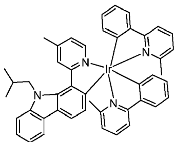
Compound 34
