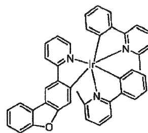
Compound 6
