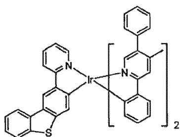
Compound 63
