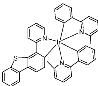
Compound 16
