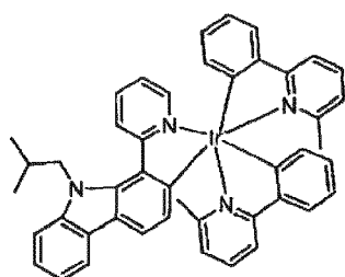
Compound 28
