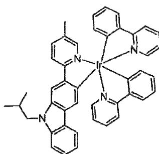
Compound 104
