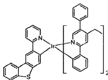
Compound 72
