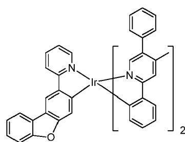
Compound 39
