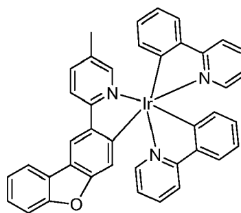
Compound 57
