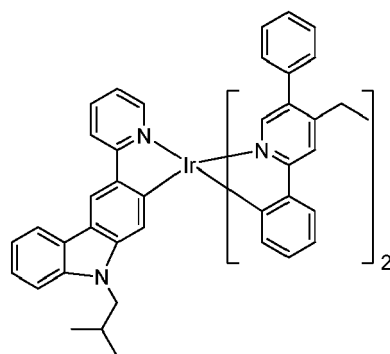
Compound 96
