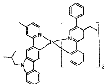
Compound 98
