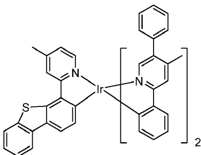
Compound 64
