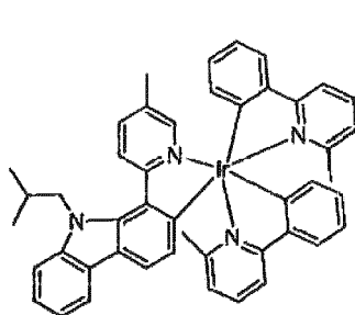
Compound 106
