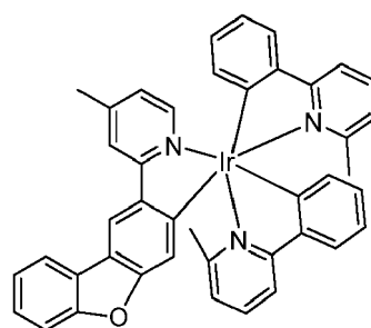
Compound 12
