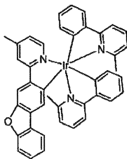
Compound 11
