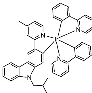
Compound 33
