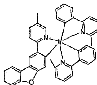
Compound 60
