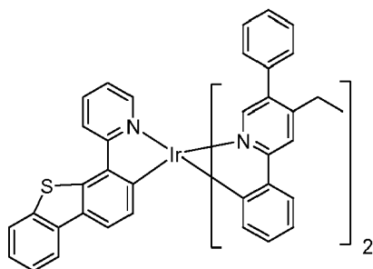
Compound 70
