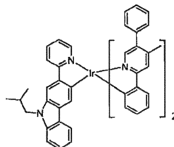
Compound 86
