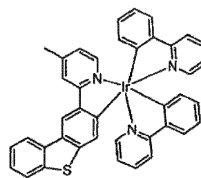
Compound 21
