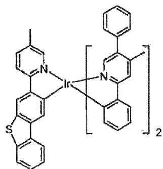
Compound 68
