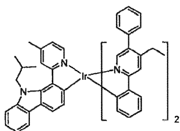
Compound 97
