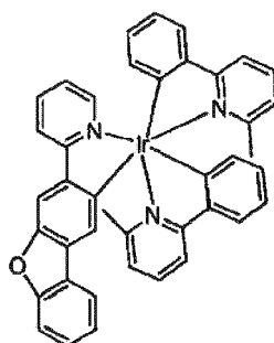
Compound 5
