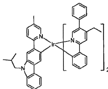
Compound 101
