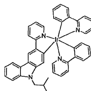
Compound 27
