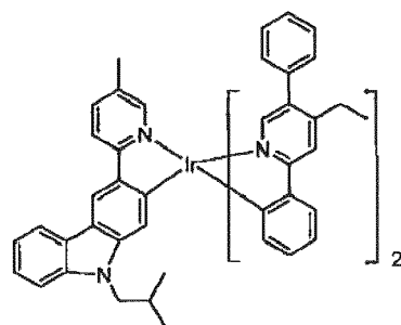
Compound 102
