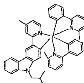
Compound 36
