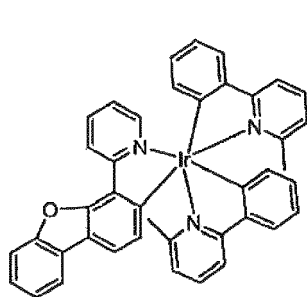
Compound 4
