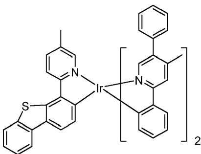
Compound 67
