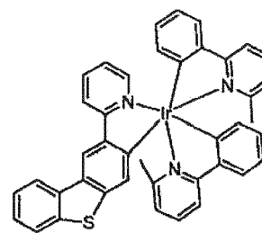
Compound 18
