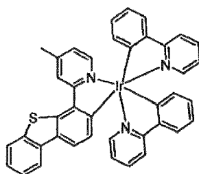
Compound 19
