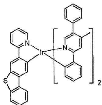
Compound 62
