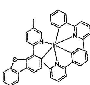
Compound 82
