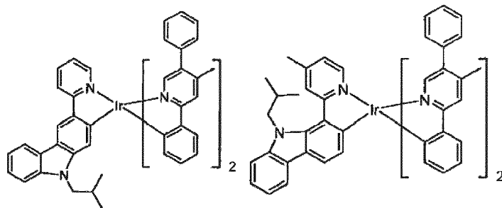
Compound 87
