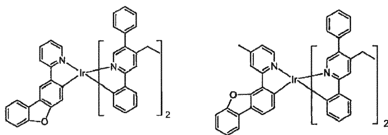
Compound 48
