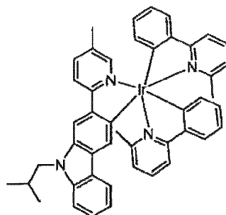
Compound 107
