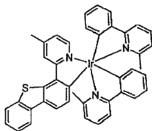
Compound 22
