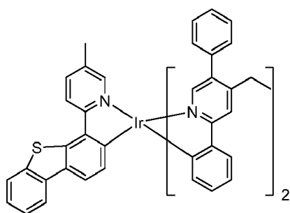
Compound 76
