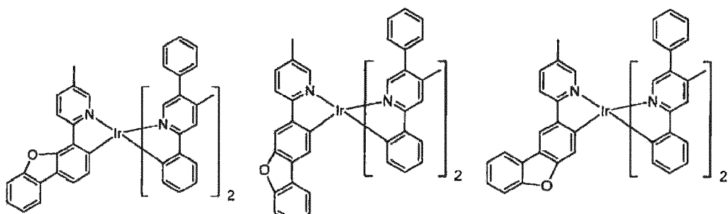
Compound 43
