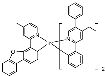
Compound 49
