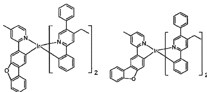
Compound 50
