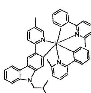
Compound 108
