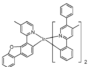
Compound 40
