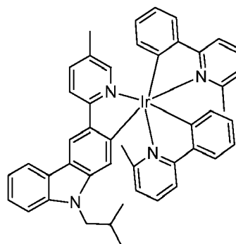
Compound 108
