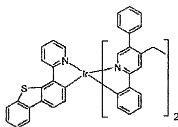
Compound 70
