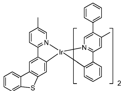
Compound 69
