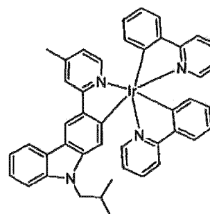
Compound 33
