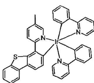
Compound 79
