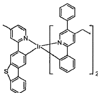
Compound 74
