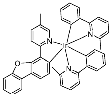
Compound 58
