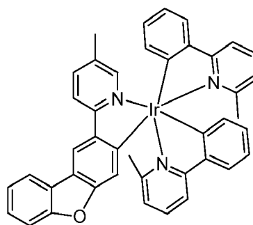
Compound 60
