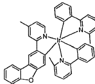
Compound 12
