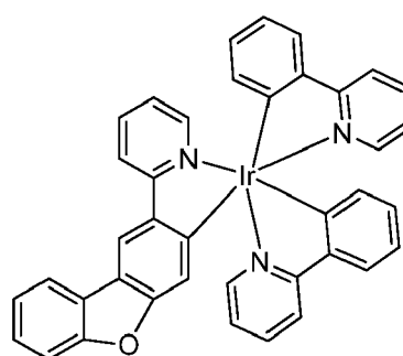
Compound 3
