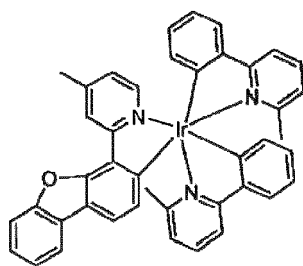
Compound 10
