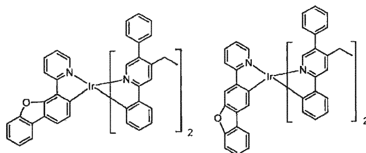
Compound 46
