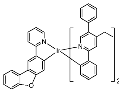
Compound 48
