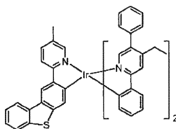
Compound 78
