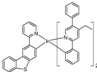
Compound 72
