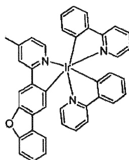
Compound 8
