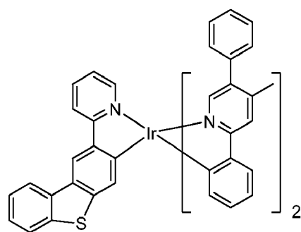
Compound 63
