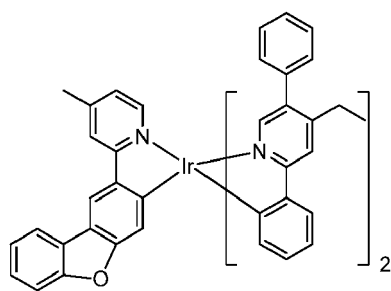
Compound 51
