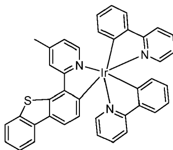
Compound 19
