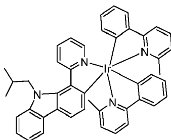
Compound 28
