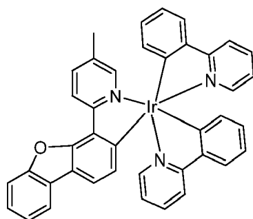
Compound 55
