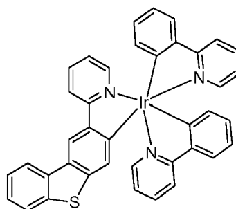
Compound 15
