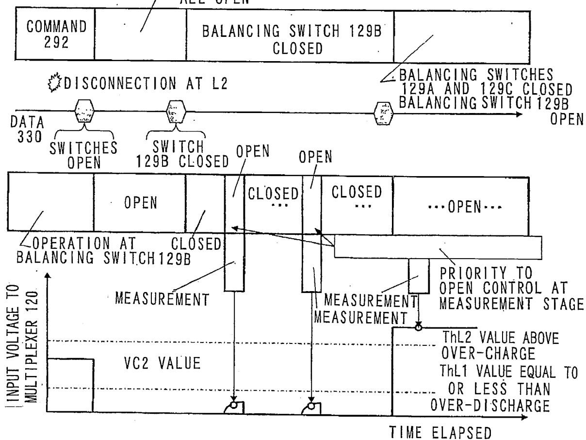
FIG.29 BALANCING SWITCHES 129 ALL OPEN
