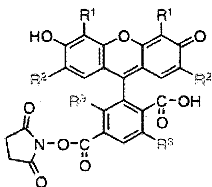
6 Structures of 6-JOE SE (C6171MP), 6-HEX SE (C20091) and 6-TET SE (C20092).
