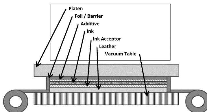
Print Cross Section
