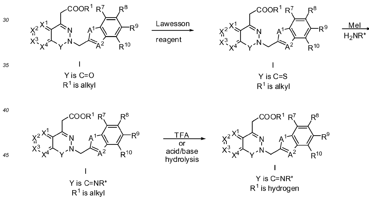
Scheme 11.
