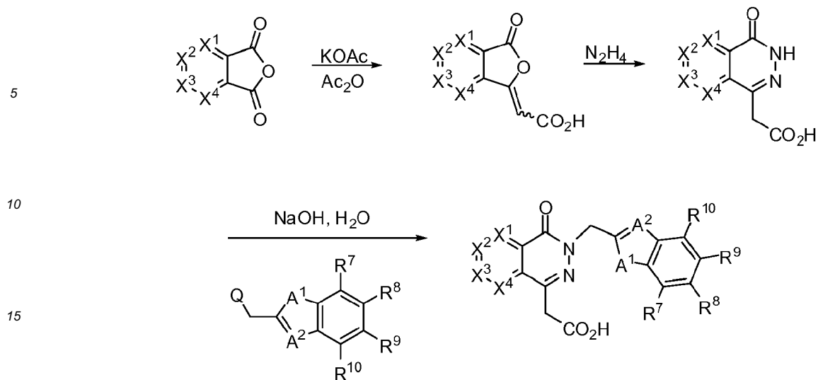
Scheme 13.
