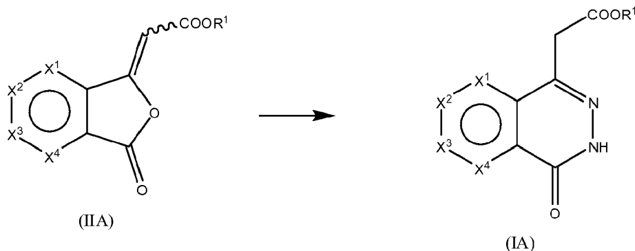
Scheme 5.
