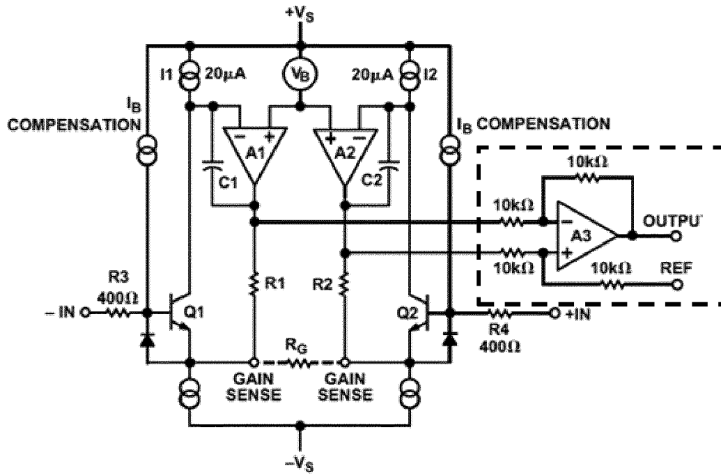
FIG 29 (prior art)
