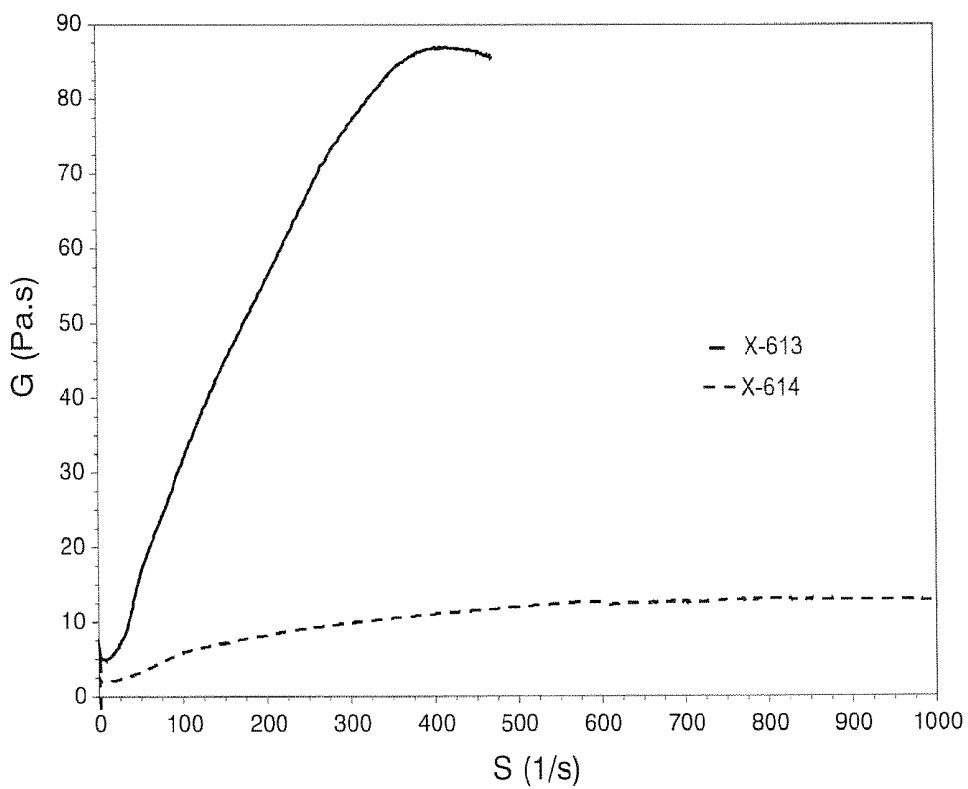
FIG. 7 -- 4-Week Shear Viscosity
