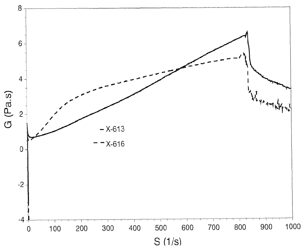
FIG. 12 -- 1-Day Shear Viscosity
