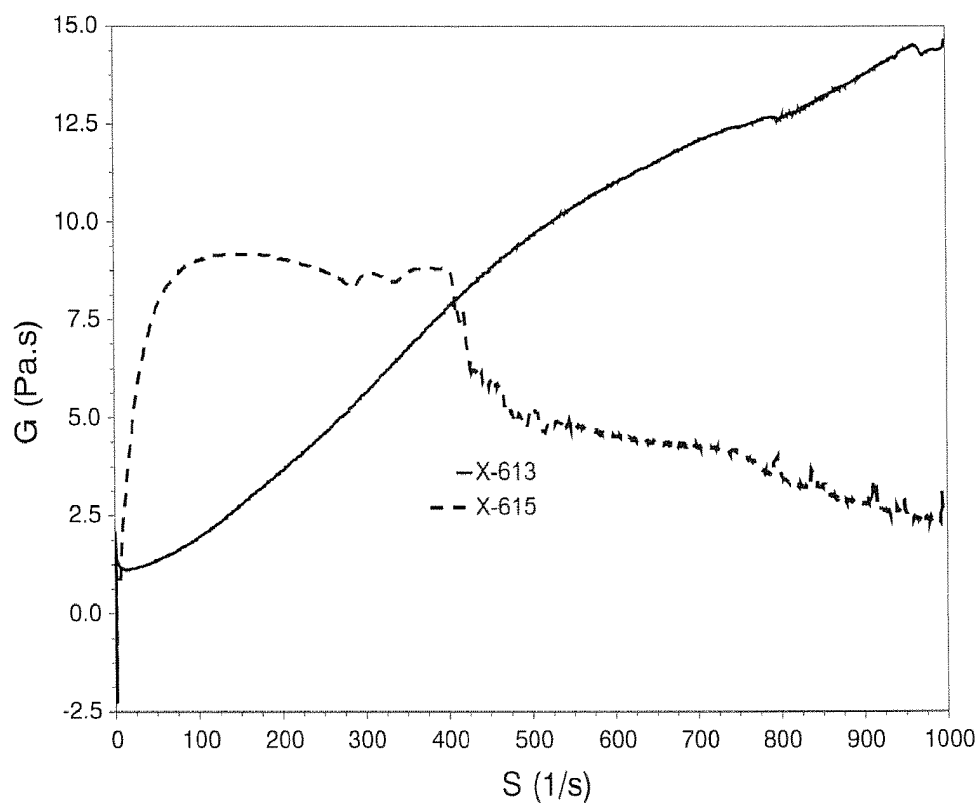
FIG. 19 -- 3-Day Shear Viscosity
