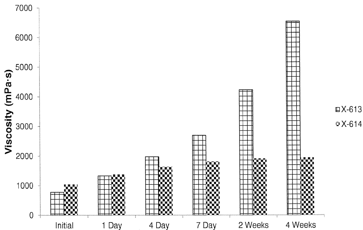
FIG. 1 -- Brookfield Viscosity Data
