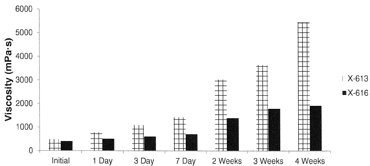
FIG. 10 -- Brookfield Viscosity Data
