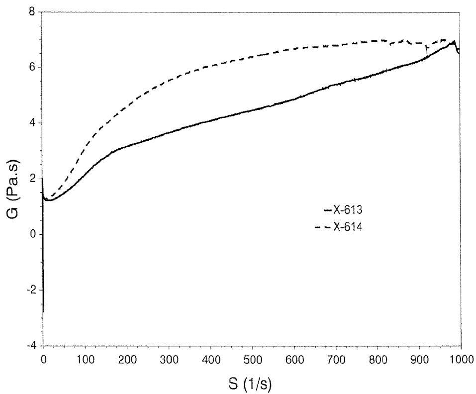
FIG. 4 -- 1-Day Shear Viscosity
