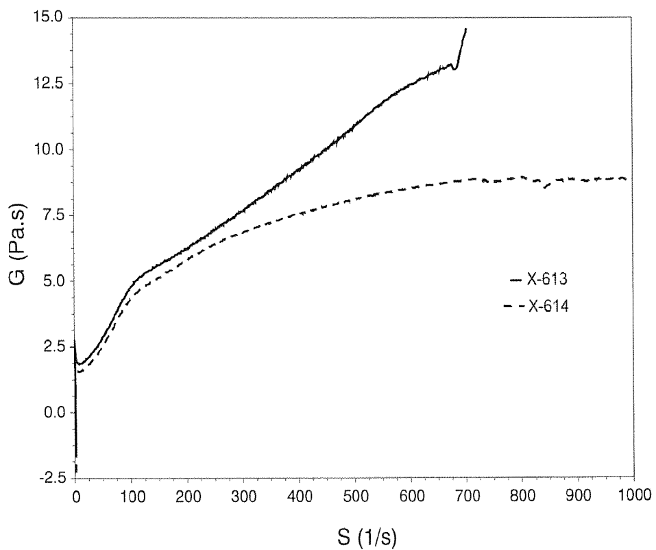
FIG. 5 -- 4-Day Shear Viscosity
