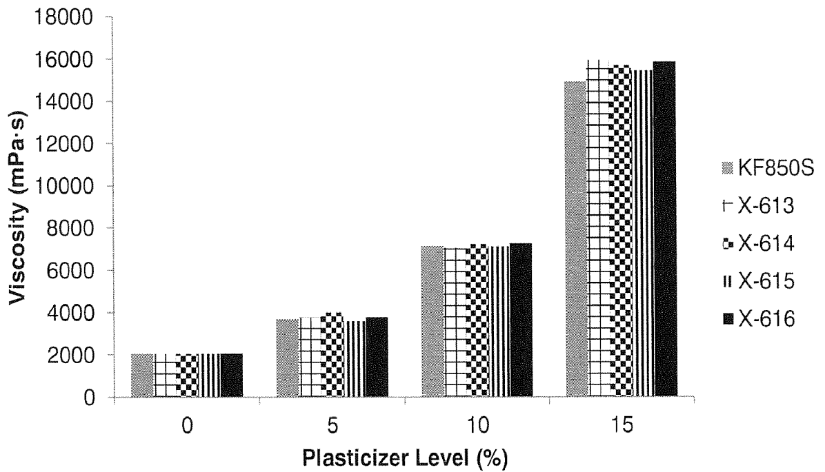
FIG. 26 -- 7-Day Viscosity Response - Copolymer
