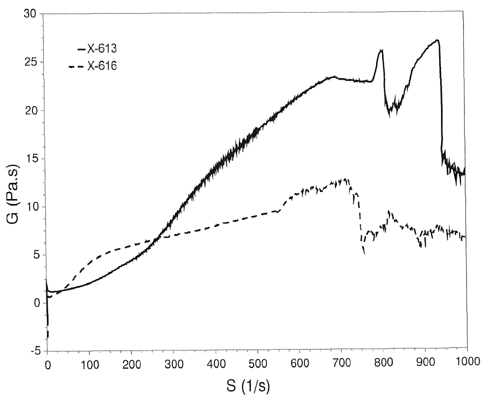
FIG. 14 -- 7-Day Shear Viscosity
