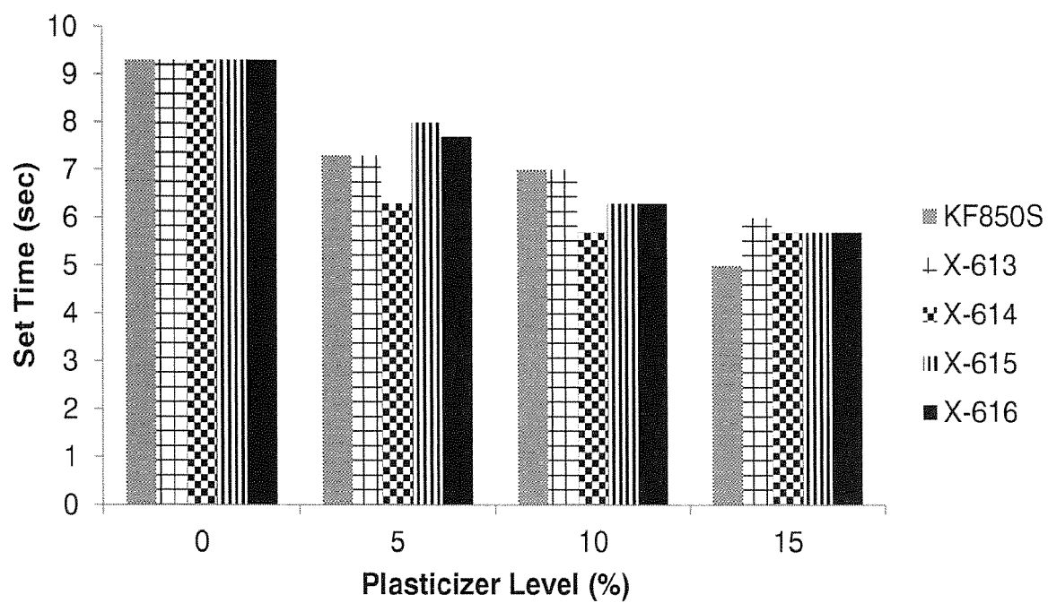
FIG. 28 -- Copolymer Set Times
