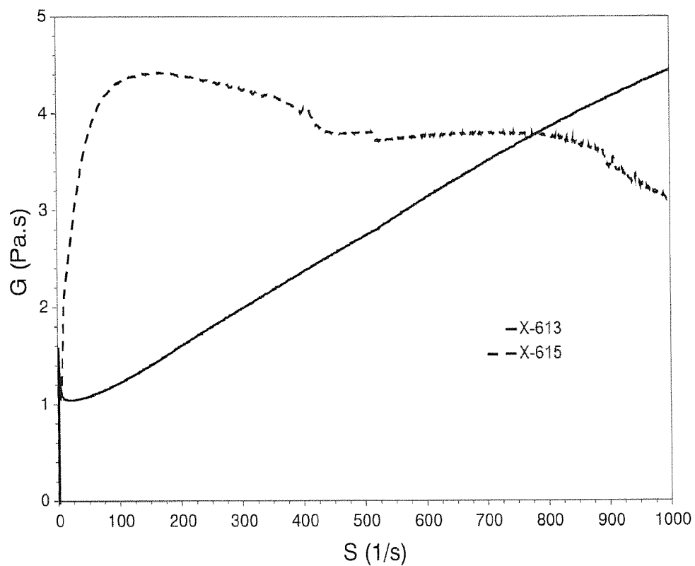
FIG. 17 -- Initial Shear Viscosity
