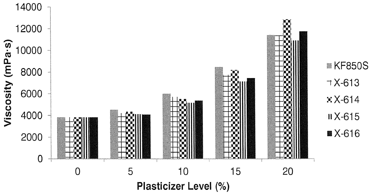
FIG. 32 -- 3-Day Viscosity Response - Homopolymer
