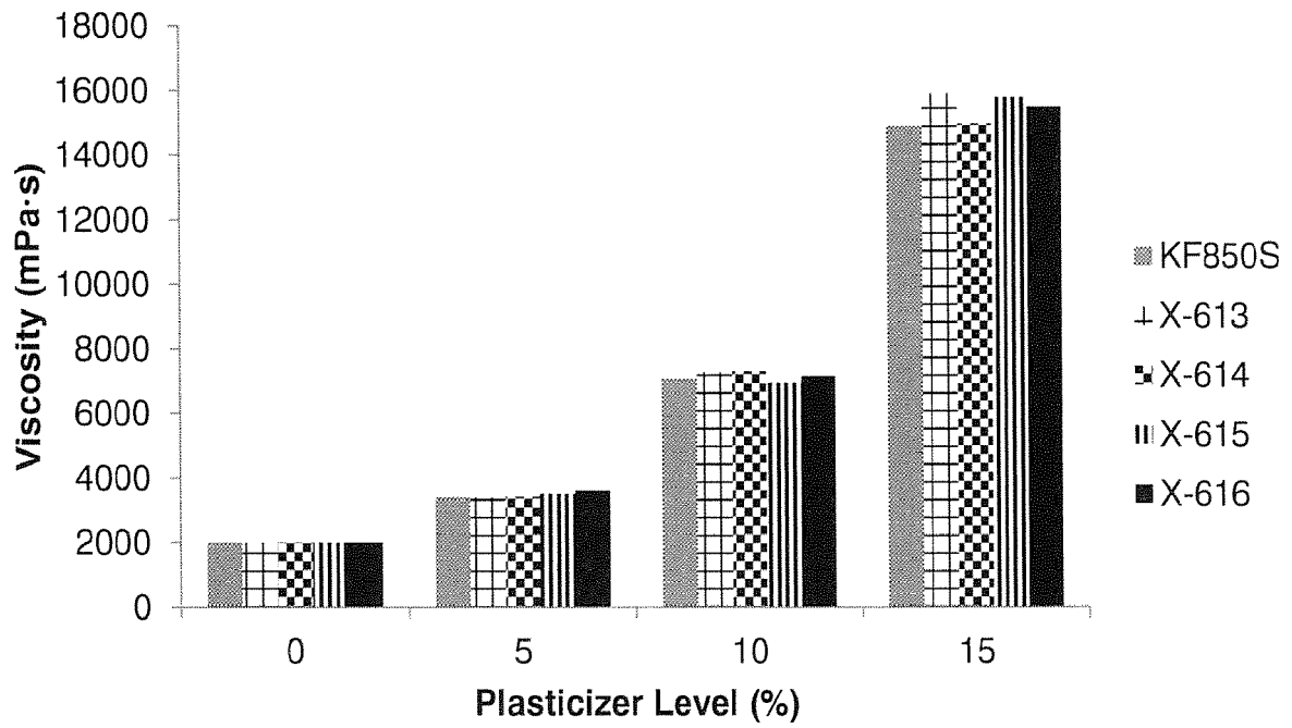
FIG. 23 -- Initial Viscosity Response - Copolymer
