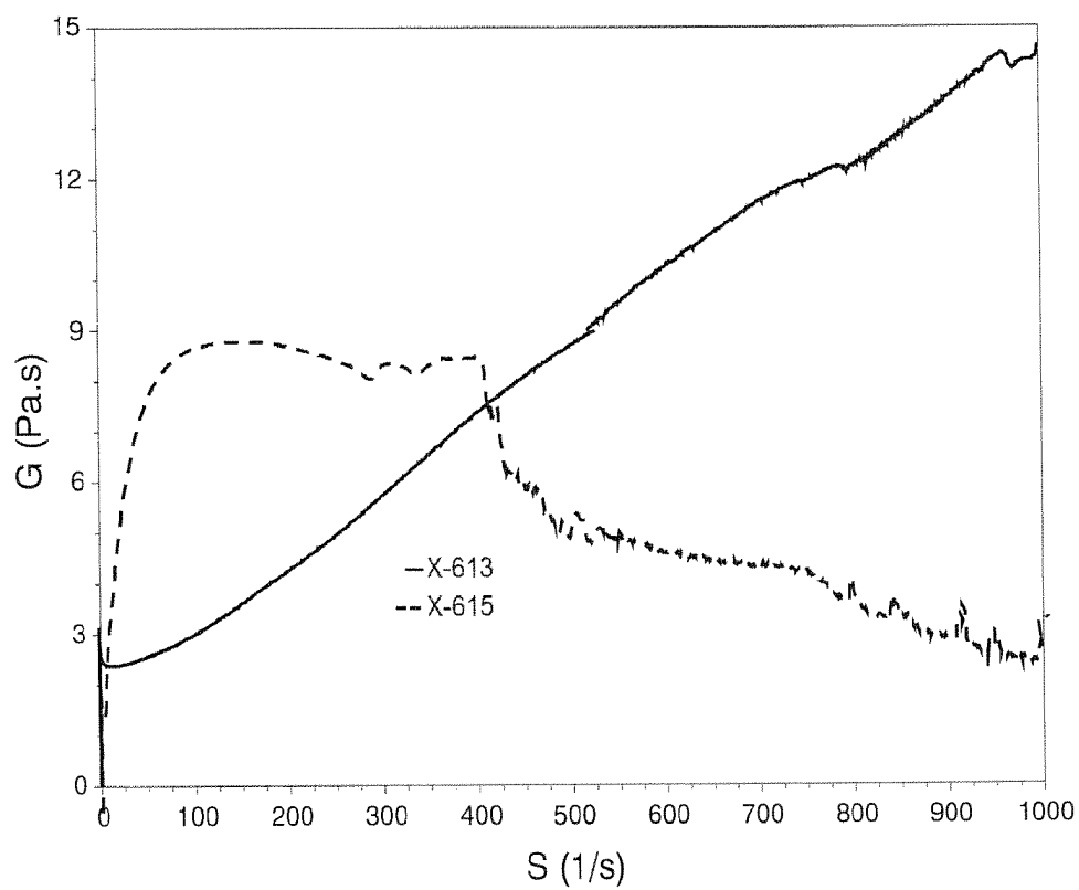
FIG. 18 -- 1-Day Shear Viscosity
