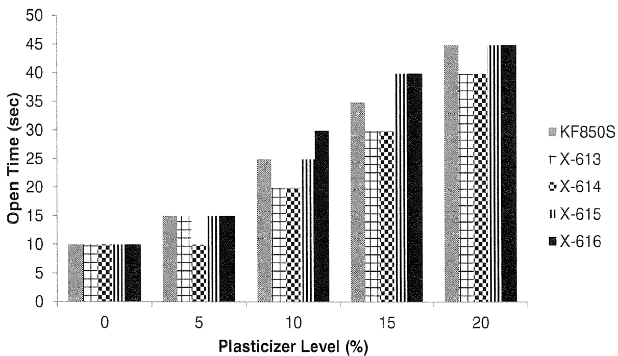
FIG. 36 -- Open Times - Homopolymer
