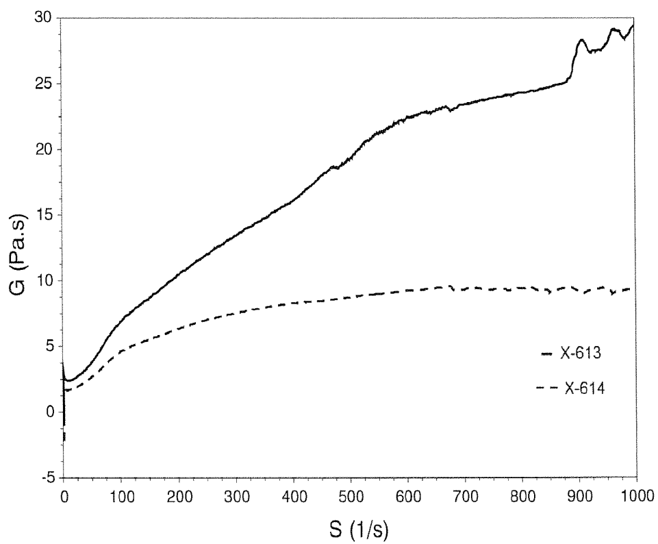
FIG. 6 -- 7-Day Shear Viscosity
