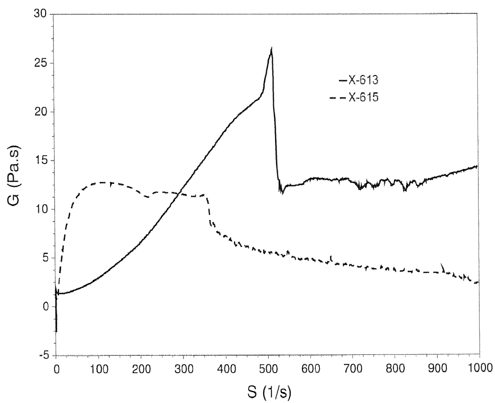
FIG. 20 -- 7-Day Shear Viscosity
