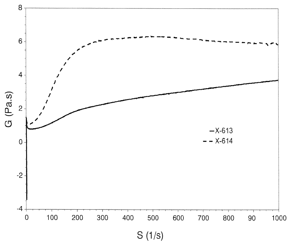
FIG. 3 -- Initial Shear Viscosity
