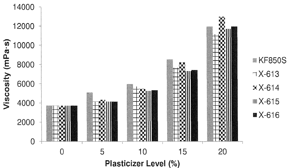
FIG. 31 -- 1-Day Viscosity Response - Homopolymer
