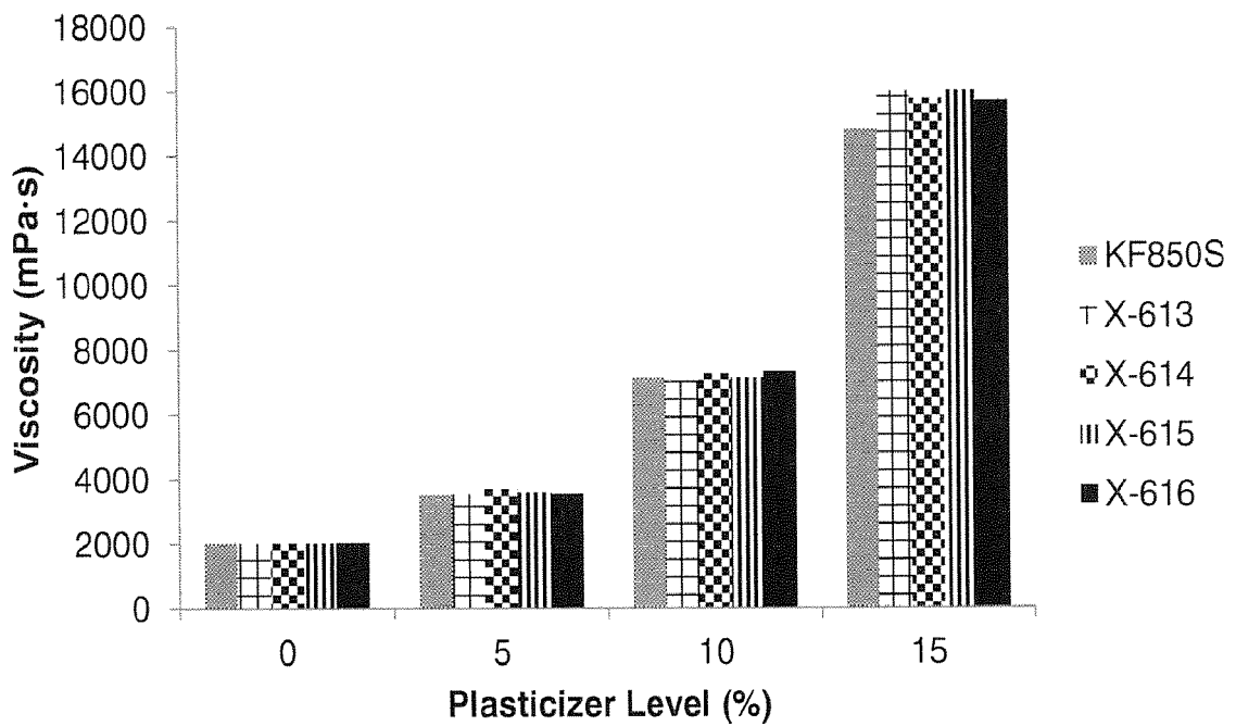
FIG. 24 -- 1-Day Viscosity Response - Copolymer
