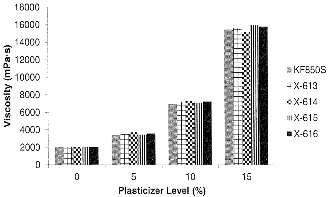
FIG. 25 -- 3-Day Viscosity Response - Copolymer
