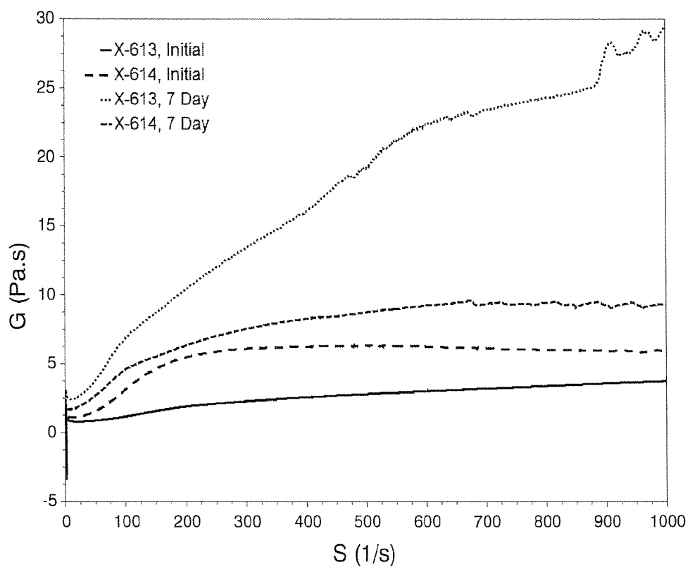
FIG. 8 -- Initial vs. 7-Day Shear
