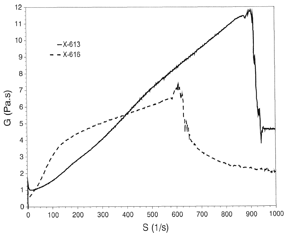
FIG. 13 -- 3-Day Shear Viscosity
