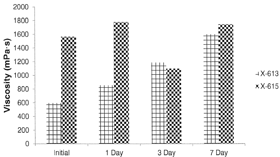
FIG. 16 -- Brookfield Viscosity Data
