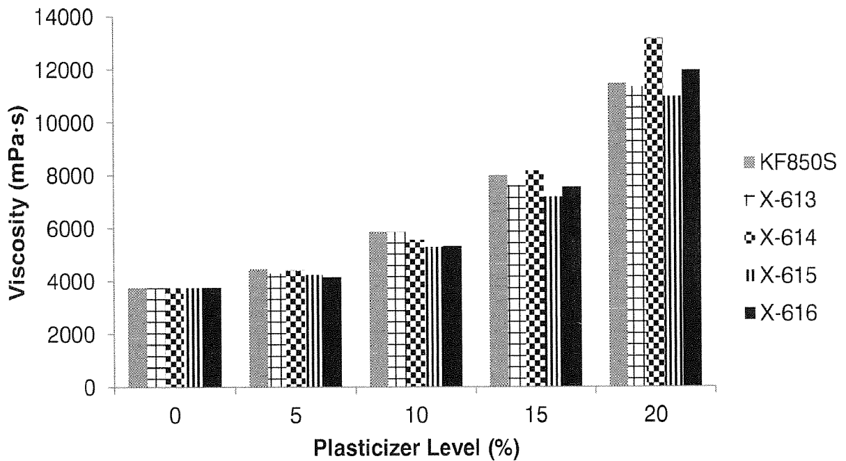
FIG. 33 -- 7-Day Viscosity Response - Homopolymer
