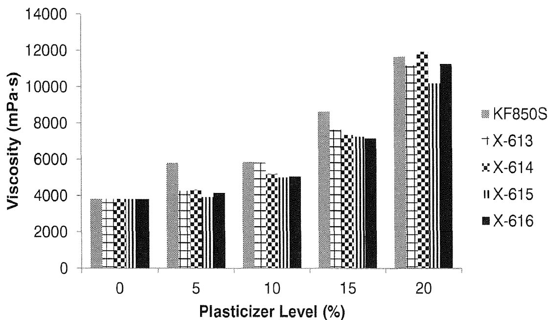
FIG. 30 -- Initial Viscosity Response - Homopolymer
