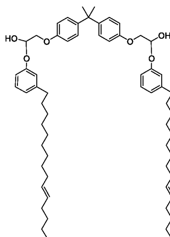
Molecular Structure 1
