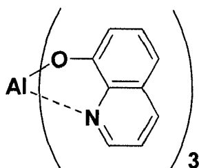
ET-1 ( \text{Alq}_3 )
