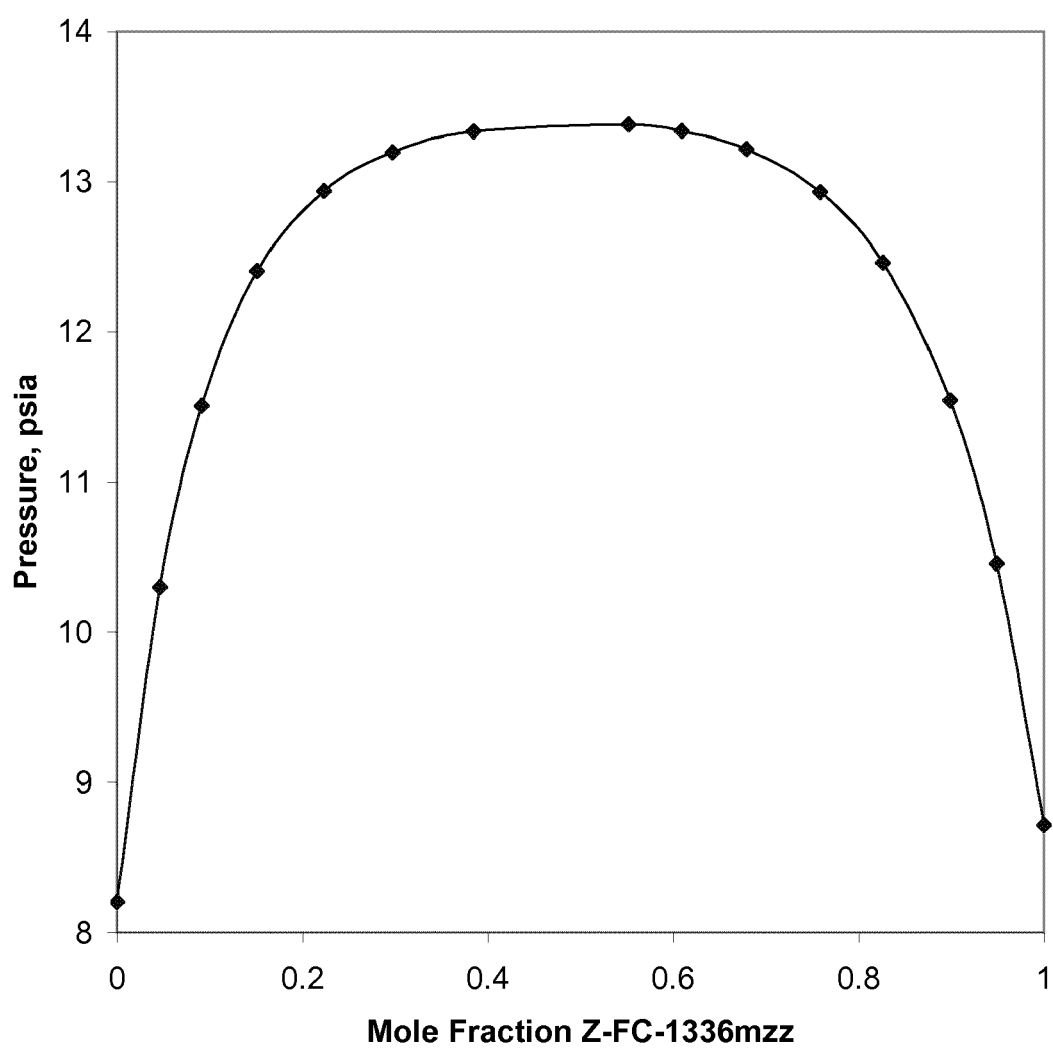
FIGURE 2. Z-FC-1336mzz and n-Pentane at 19.9 C
