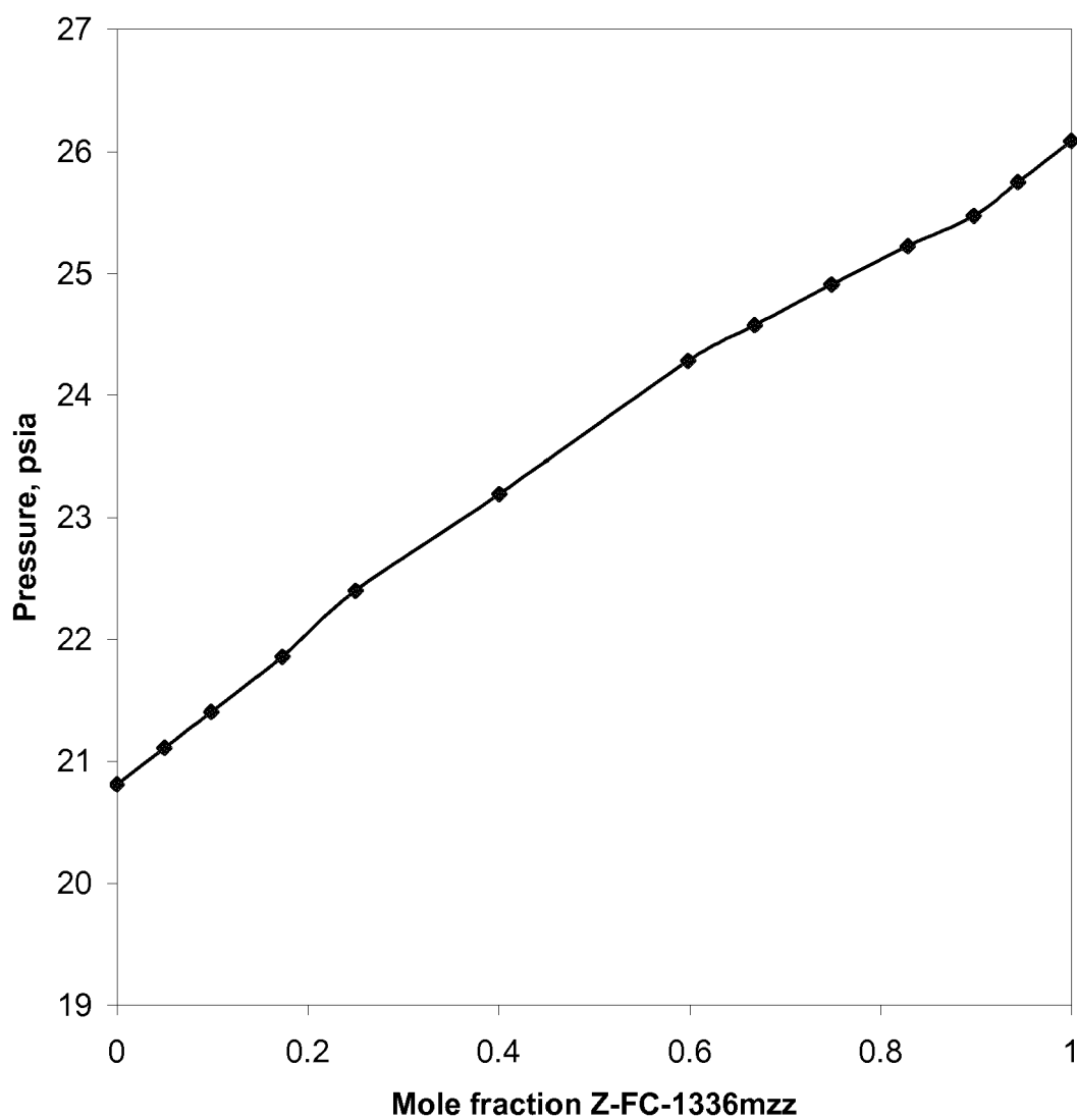
FIG. 4 - Z-FC-1336mzz and HFC-365mfc at 50.1 C
