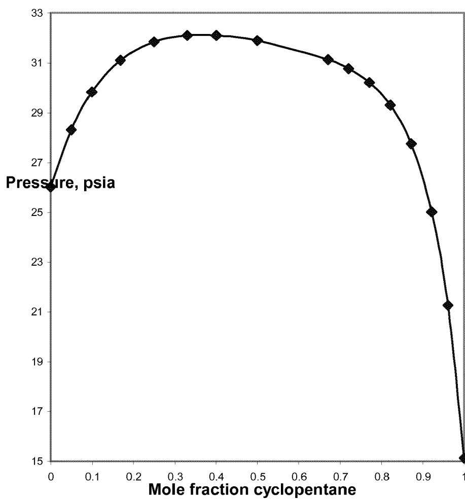
FIG. 1 - Z-FC-1336mzz and Cyclopentane at 50 C
