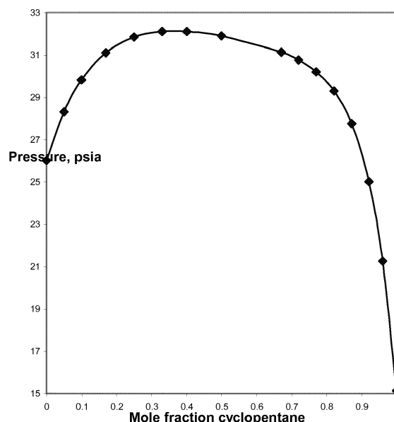
FIG. 1 - Z-FC-1336mzz and Cyclopentane at 50 C
