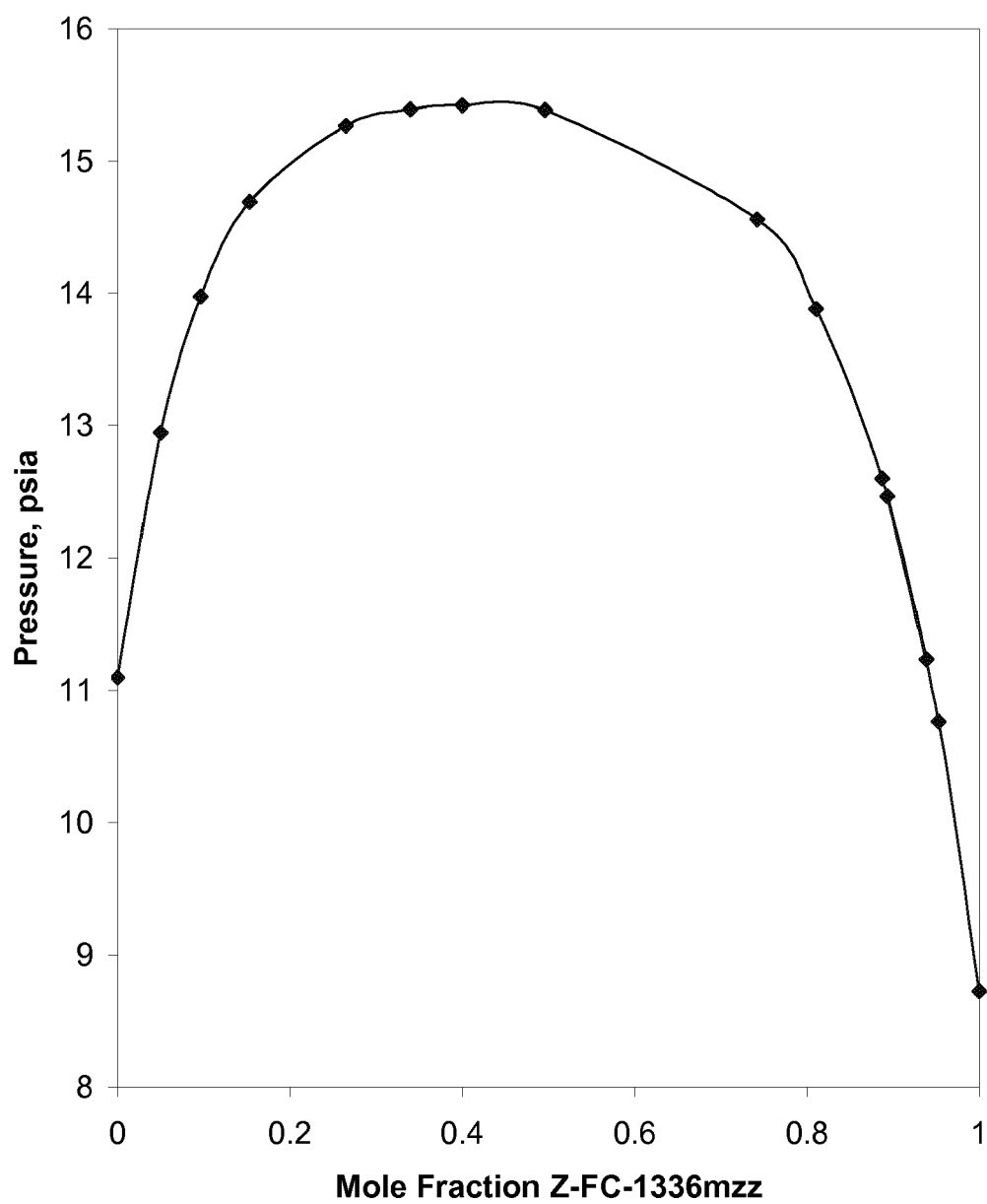
FIGURE 3. Z-FC-1336mzz and Isopentane at 19.9 C
