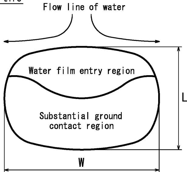
Ground contact configuration of wide-width tire
