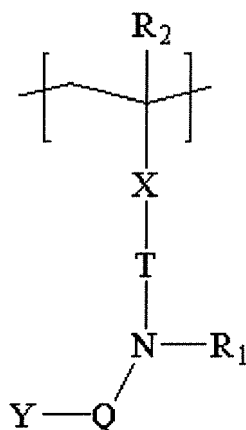
[Structural Formula 4]
