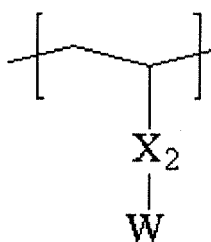
[Structural Formula 7]
