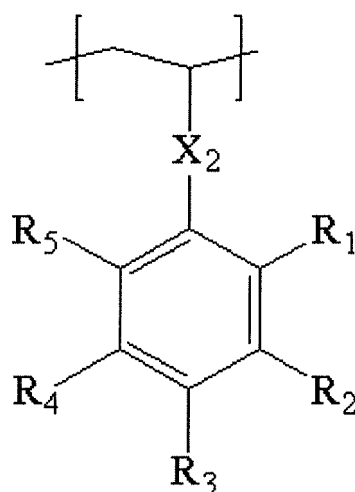
[Structural Formula 3]
