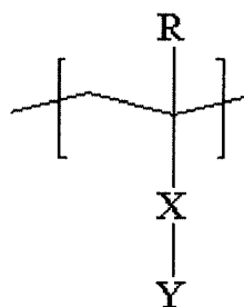
[Structural Formula 3]
