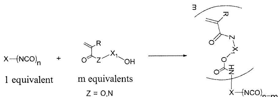
Synthesis Scheme 4
