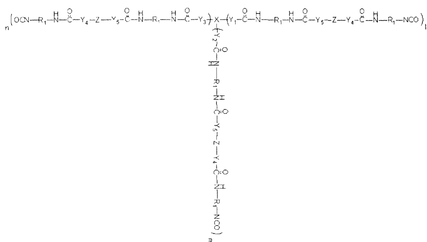
Synthesization Scheme 2
