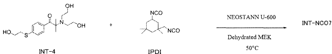
Synthesis Scheme 3
