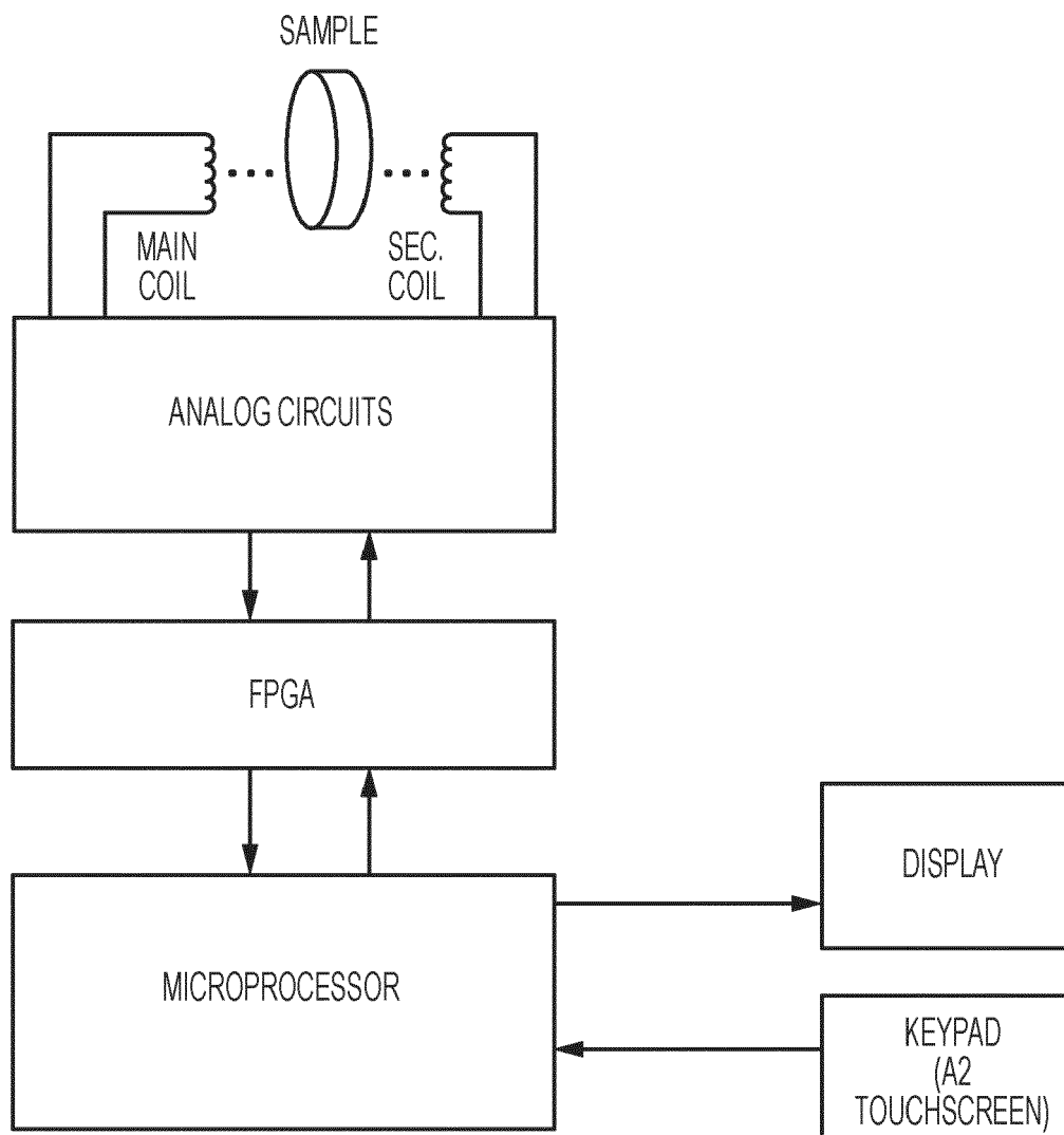
OVERALL SYSTEM ARCHITECTURE
