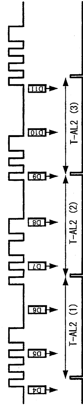
FIG. 17A Rx STA-0 Tx STA-0 State Trigger
