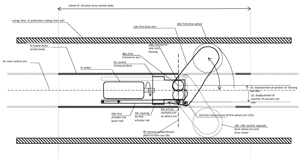
Figure 1 Parallel arranged arms, mutually displaced wheel arm transverse bearings mutually oppositely displaced actuator rods
