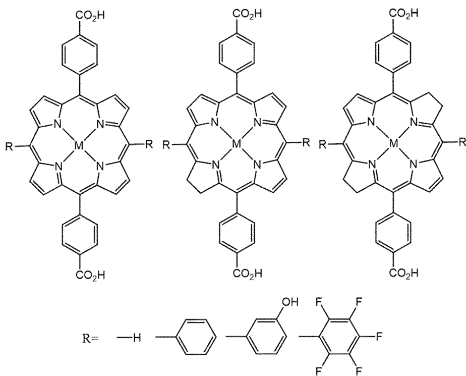
Scheme 1. Exemplary DBP, DBC, and DBBC ligands.
