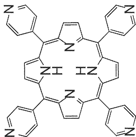
5,10,15,20-tetra(p-pyridyl)porphyrin
