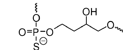
1,2,4-Butanetriol Linker
