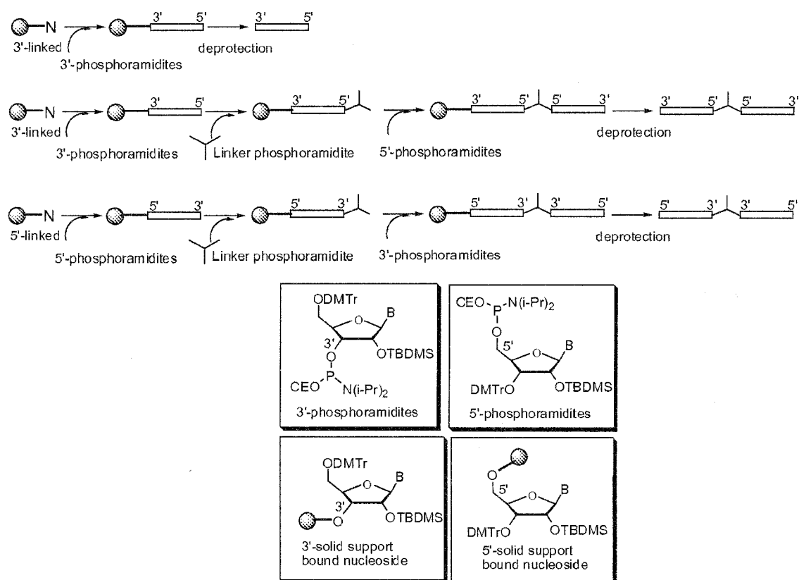
Figure 1. Linear synthesis of immune regulatory oligonucleotides.
