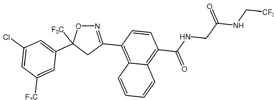
Compound A
