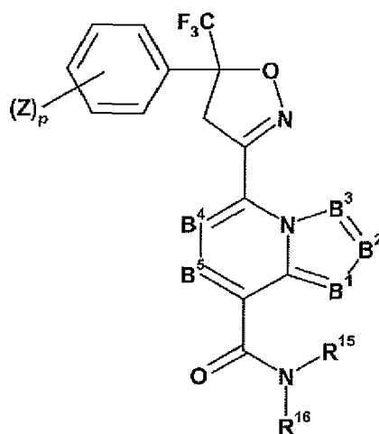
Formula (III)
