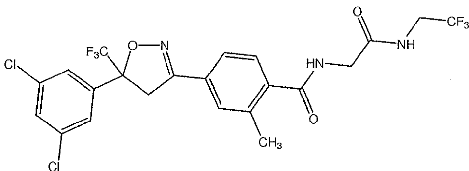
Compound B
