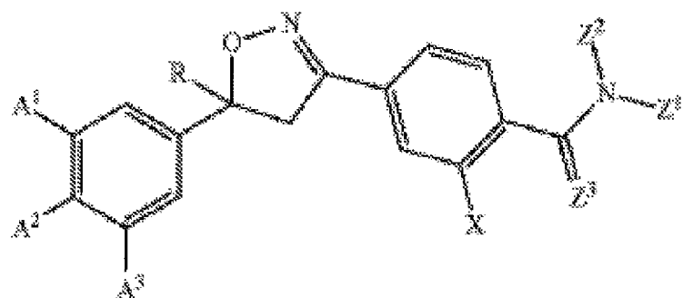
Formula (II)
