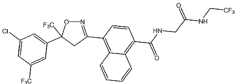
Compound A
