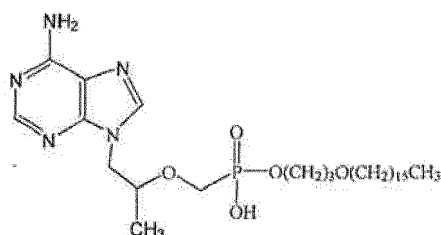
Compound I
