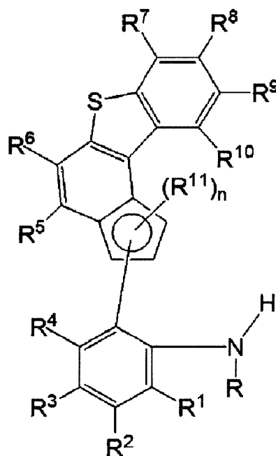
[Chemical Formula 2]
