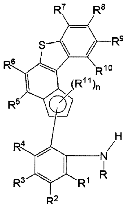
[Chemical Formula 2]
