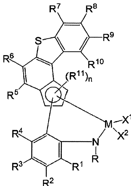
[Chemical Formula 1]
