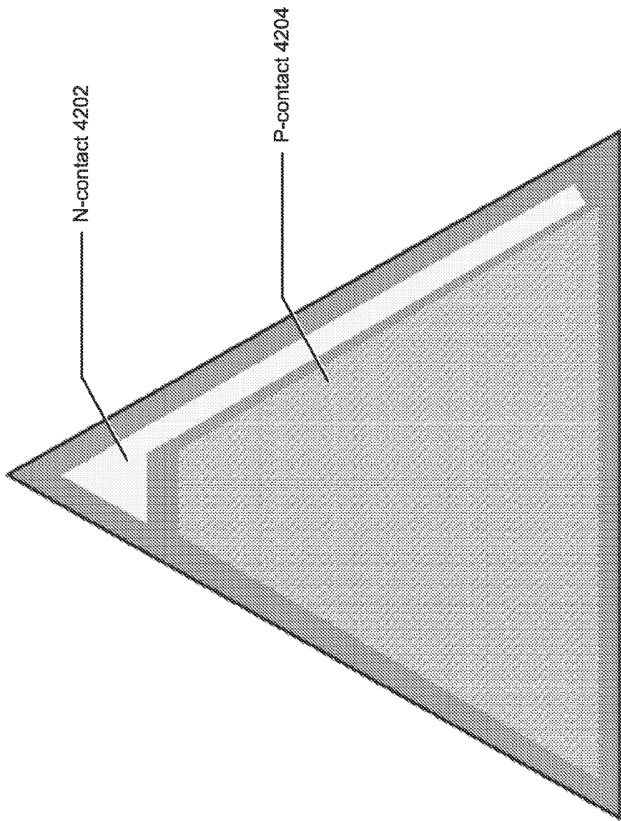
Die design with single edge corner n-contact and bus bar along one edge.
