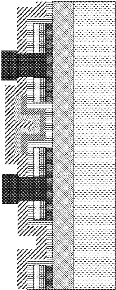
Dielectric Structure
