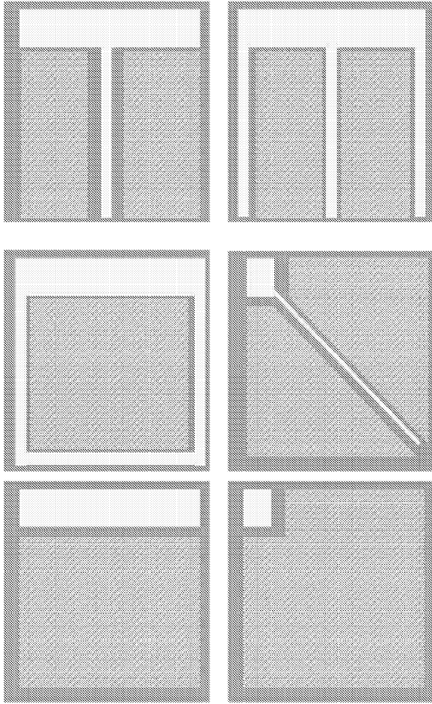
Square or rectangular die with various n- and p-contact patterns. The area can split between n and p contacts many ways (with different shapes of pads and including ring, bus-bar, and/or interdigitated contacts) with the goal of limiting die series resistance while maximizing the area of the p-contact.
