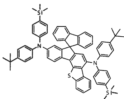
[Chemical Formula 136]
