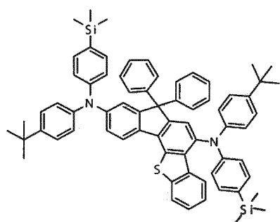
[Chemical Formula 146]
