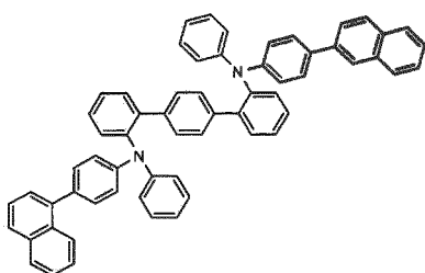
[Chemical Formula 121]
