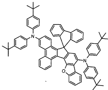
[Chemical Formula 282]
