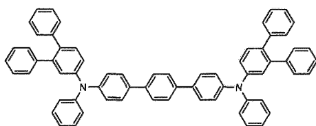
[Chemical Formula 278]
