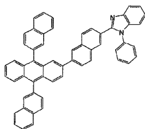
[Chemical Formula 188]
