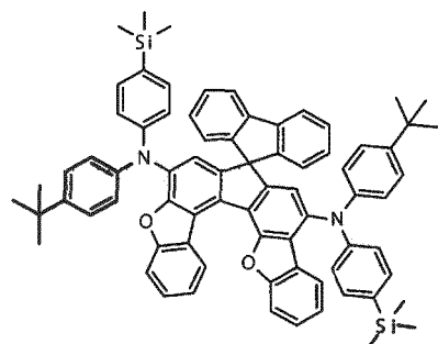
[Chemical Formula 152]
