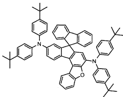
[Chemical Formula 284]
