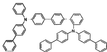
[Chemical Formula 53]
