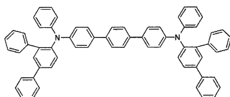
[Chemical Formula 106]
