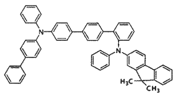
[Chemical Formula 55]
