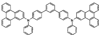
[Chemical Formula 48]
