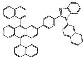
[Chemical Formula 187]
