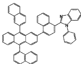
[Chemical Formula 185]
