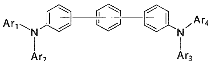
[Chemical Formula 1]
