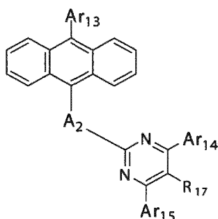
[Chemical Formula 6]
