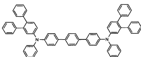
[Chemical Formula 124]
