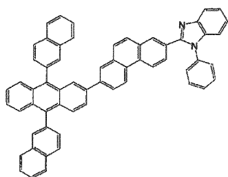
[Chemical Formula 189]
