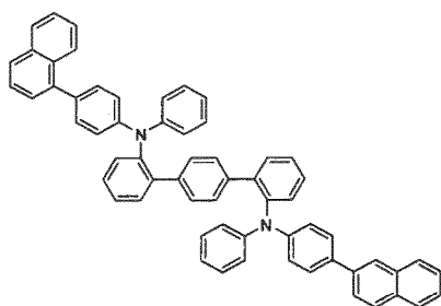
[Chemical Formula 79]
