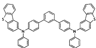
[Chemical Formula 41]
