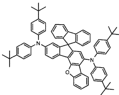
[Chemical Formula 281]
