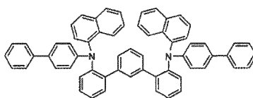
[Chemical Formula 63]
