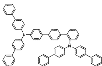
[Chemical Formula 54]
