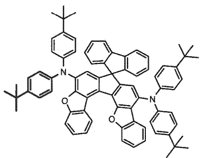
[Chemical Formula 150]
