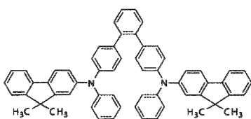
[Chemical Formula 61]
