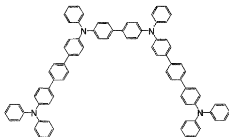
[Chemical Formula 247]
