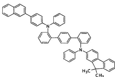
[Chemical Formula 77]
