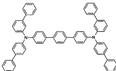
[Chemical Formula 110]
