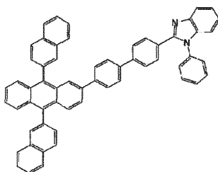
[Chemical Formula 176]
