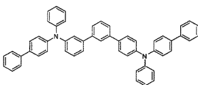
[Chemical Formula 36]
