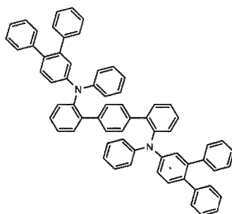
[Chemical Formula 128]
