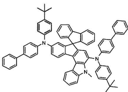
[Chemical Formula 139]
