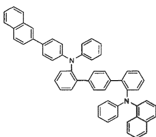
[Chemical Formula 83]
