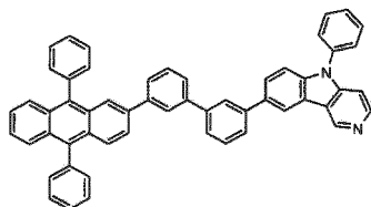
[Chemical Formula 171]
