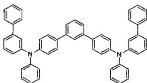
[Chemical Formula 35]
