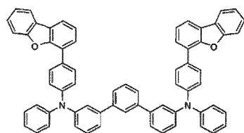
[Chemical Formula 31]
