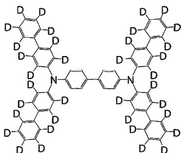
[Chemical Formula 241]
