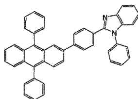
[Chemical Formula 175]
