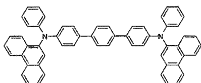
[Chemical Formula 91]
