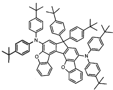
[Chemical Formula 153]
