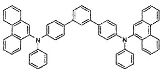
[Chemical Formula 49]
