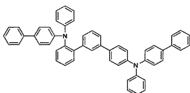
[Chemical Formula 39]
