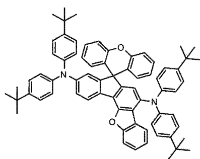
[Chemical Formula 133]
