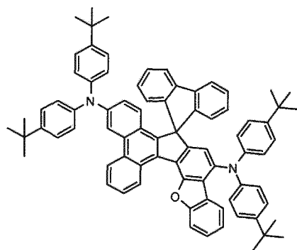
[Chemical Formula 130]
