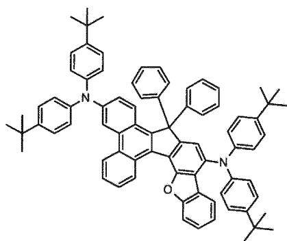
[Chemical Formula 141]
