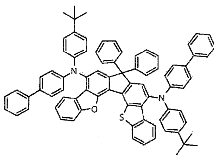
[Chemical Formula 147]
