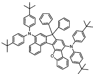
[Chemical Formula 142]
