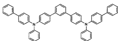
[Chemical Formula 24]
