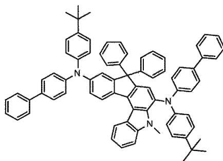
[Chemical Formula 149]
