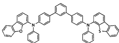
[Chemical Formula 42]
