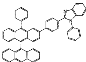
[Chemical Formula 183]
