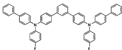
[Chemical Formula 43]
