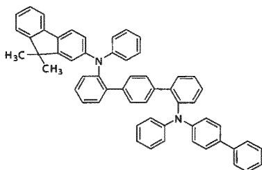
[Chemical Formula 76]
