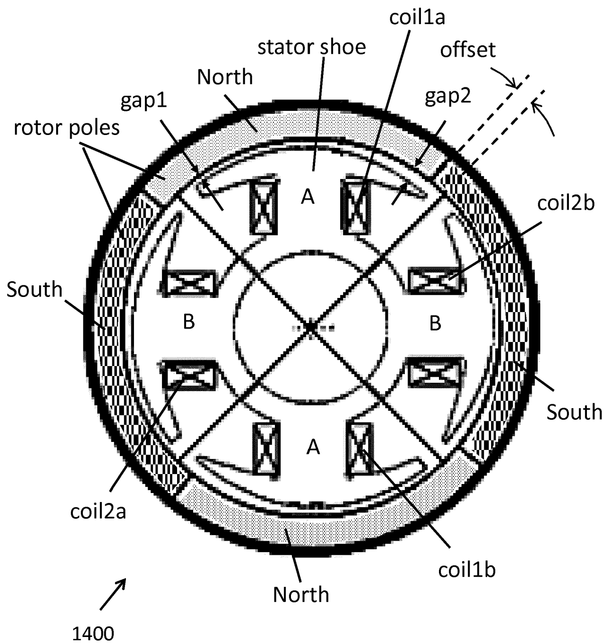
FIG. 14 (prior art)
