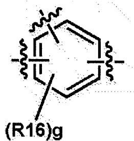
[Chemical Formula 3-3]
