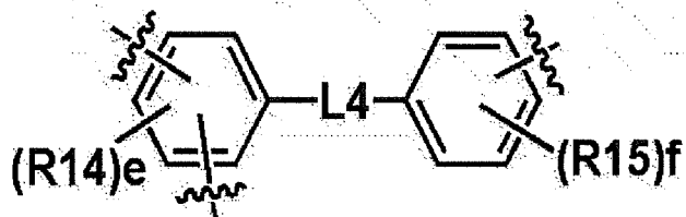
[Chemical Formula 3-3]
