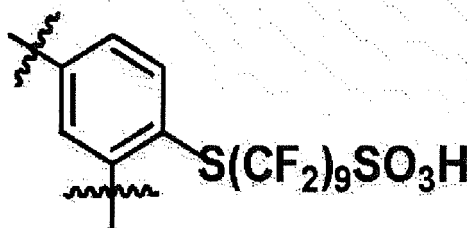
[Chemical Formula 1-9]
