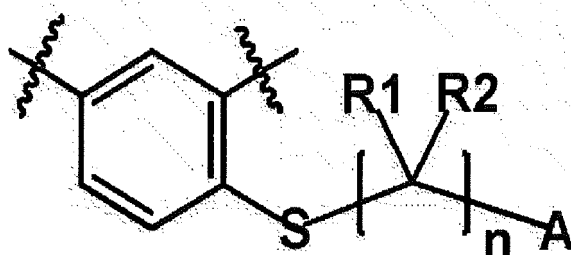
[Chemical Formula 2]
