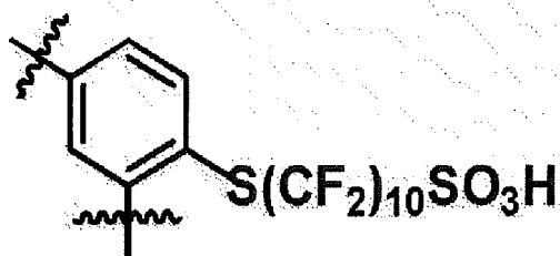
[Chemical Formula 1-9]
