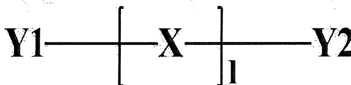
[Chemical Formula 3]
