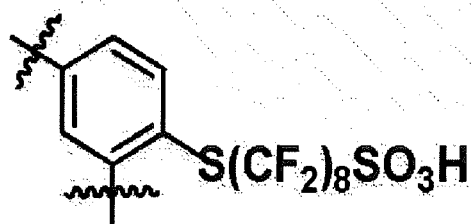
[Chemical Formula 1-7]
