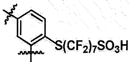
[Chemical Formula 1-7]
