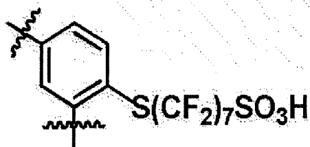
[Chemical Formula 1-6]
