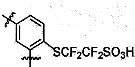
[Chemical Formula 1-2]
