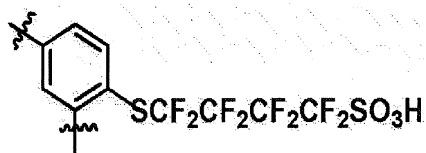
[Chemical Formula 1-4]
