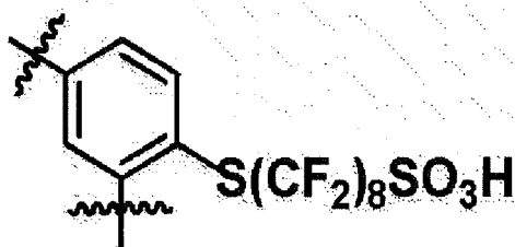
[Chemical Formula 1-8]
