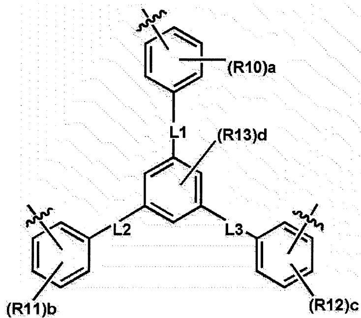
[Chemical Formula 3-2]
