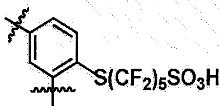
[Chemical Formula 1-5]
