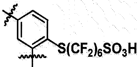
[Chemical Formula 1-6]
