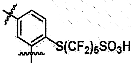
[Chemical Formula 1-5]
