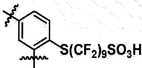
[Chemical Formula 1-9]
