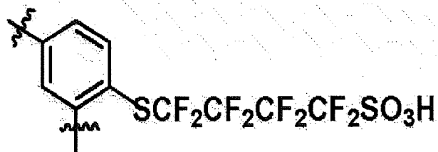
[Chemical Formula 1-4]
