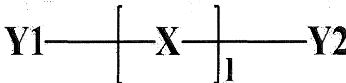
[Chemical Formula 5]
