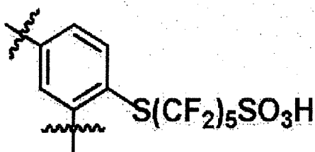
[Chemical Formula 1-5]
