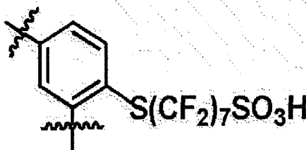
[Chemical Formula 1-7]
