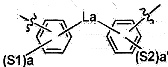
[Chemical Formula 2]
