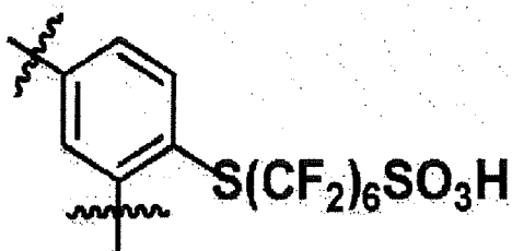
[Chemical Formula 1-5]
