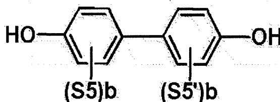
[Chemical Formula 3-4]
