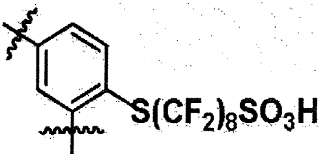
[Chemical Formula 1-8]
