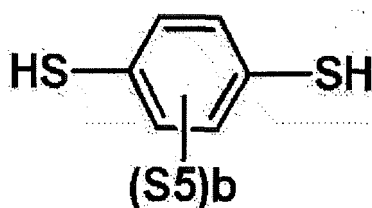
[Chemical Formula 3-3]
