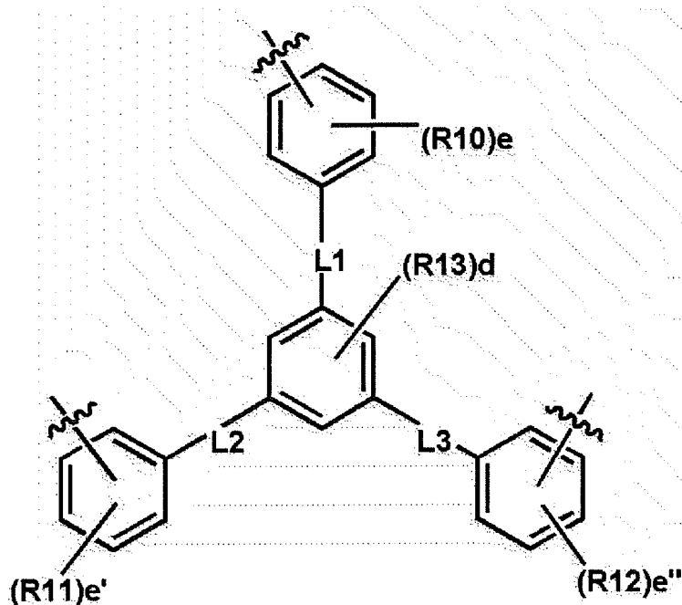
[Chemical Formula 5-1]
