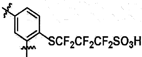
[Chemical Formula 1-2]
