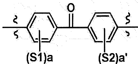
[Chemical Formula 2-2]
