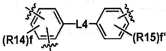
[Chemical Formula 5-3]
