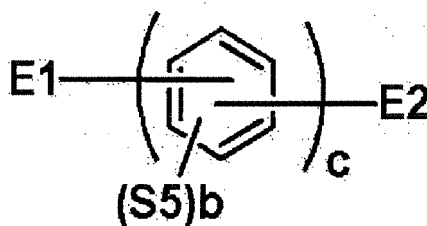
[Chemical Formula 3]
