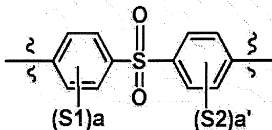
[Chemical Formula 2-2]
