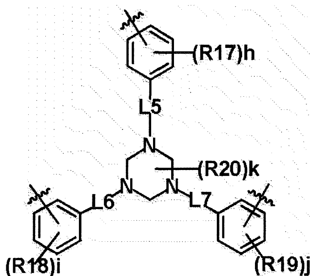
[Chemical Formula 5-4]
