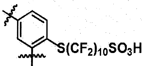
[Chemical Formula 1-9]
