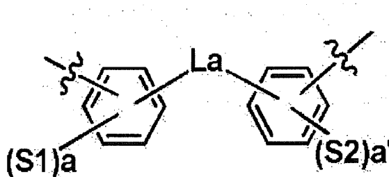
[Chemical Formula 2]
