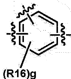
[Chemical Formula 5-3]
