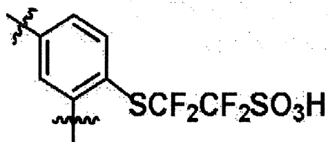
[Chemical Formula 1-2]
