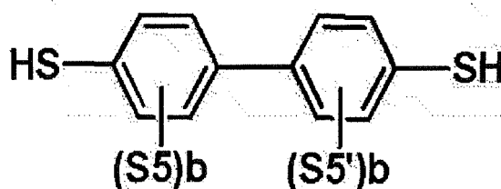
[Chemical Formula 3-4]
