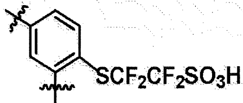
[Chemical Formula 1-2]
