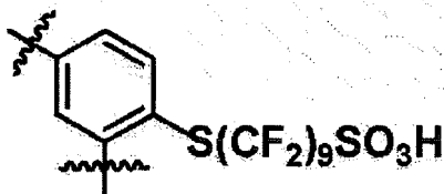
[Chemical Formula 1-9]
