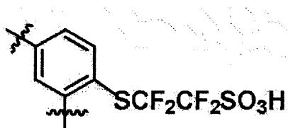
[Chemical Formula 1-2]
