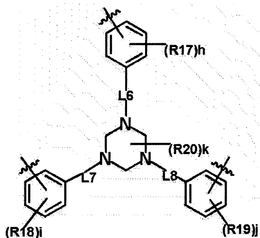
[Chemical Formula 5-4]
