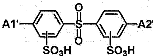
[Chemical Formula 3-1]
