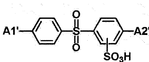
[Chemical Formula 2-3]
