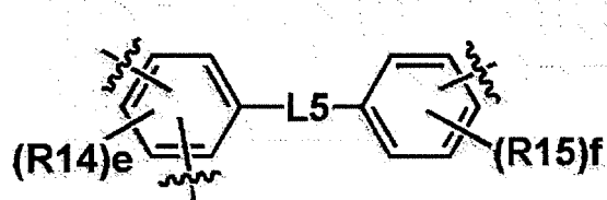
[Chemical Formula 5-3]
