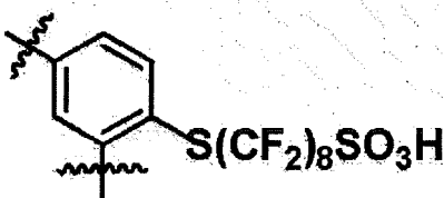
[Chemical Formula 1-8]
