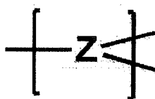
[Chemical Formula 5]
