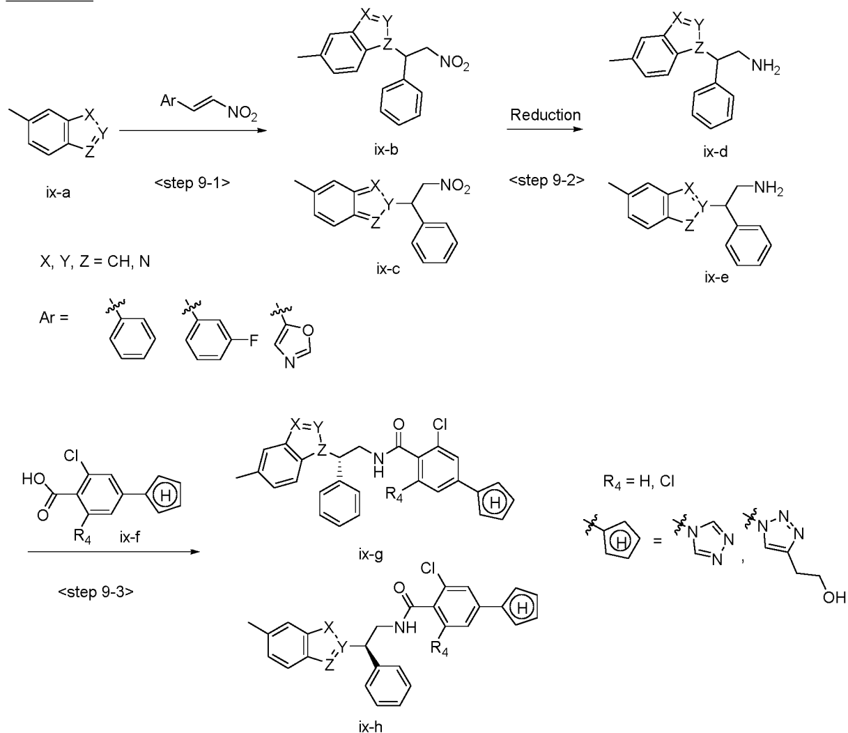
Scheme 9
