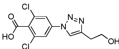
2,6-Dichloro-4-(4-(2-hydroxyethyl)-1H-1,2,3-triazol-1-yl)benzoic acid
