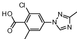
2-Chloro-6-methyl-4-(3-methyl-1H-1,2,4-triazol-1-yl)benzoic acid
