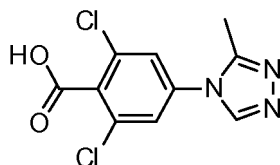
2,6-Dichloro-4-(3-methyl-4H-1,2,4-triazol-4-yl)benzoic acid
