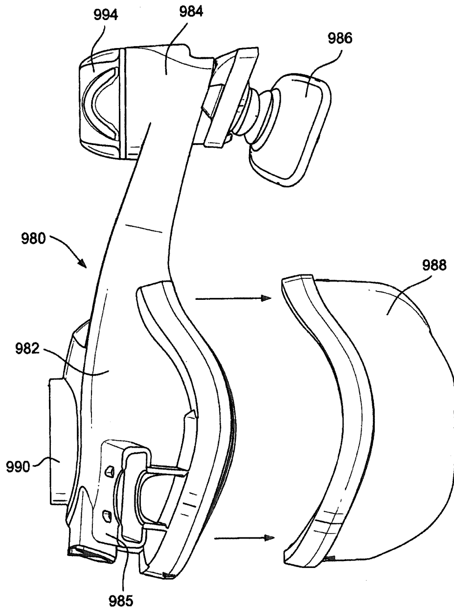
FIG. 40 (PRIOR ART)
