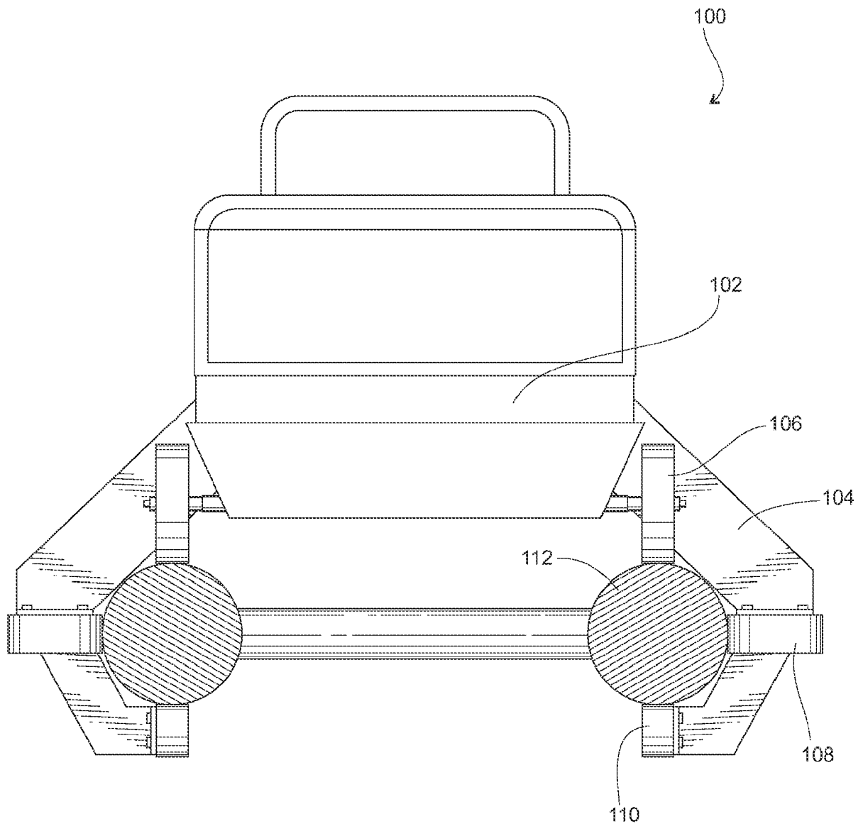
Fig. 1 PRIOR ART
