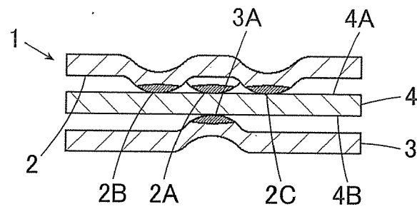
FIG. 10 PRIOR ART
