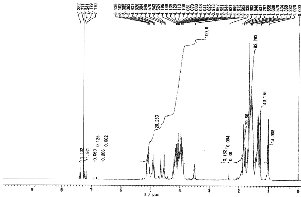
1 H-NMR SPECTRUM OF EXAMPLE 22
