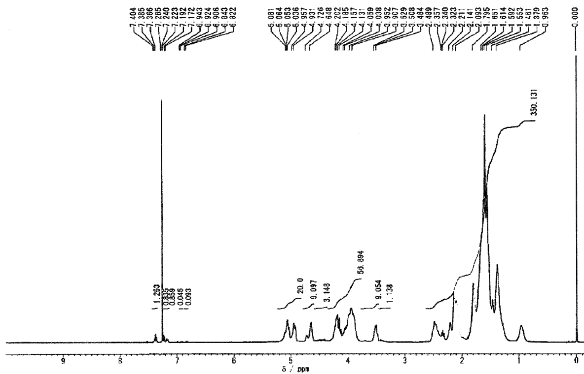
1 H-NMR SPECTRUM OF EXAMPLE 4
