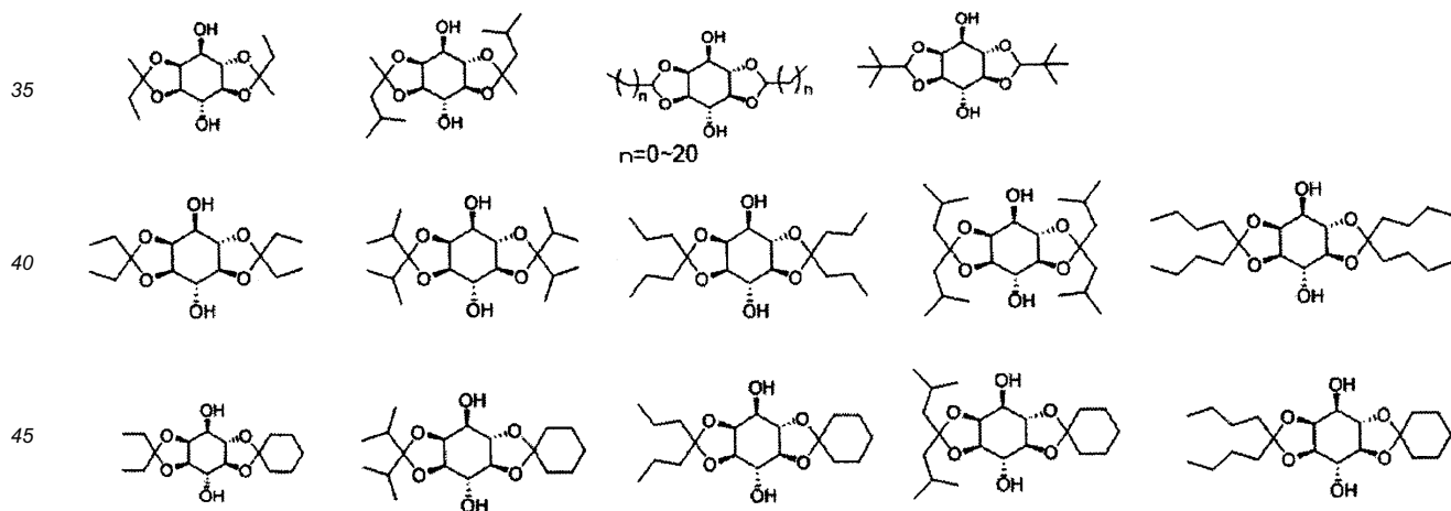
[Chem. 19]
