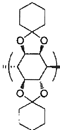
[Chem. 13]
