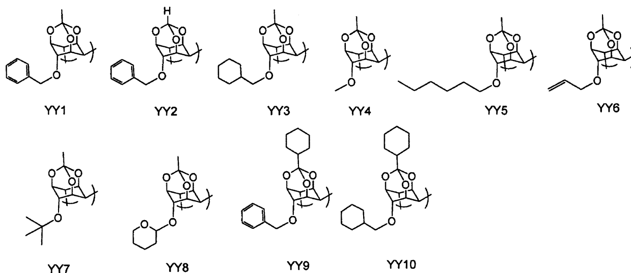
[Chem. 17]
