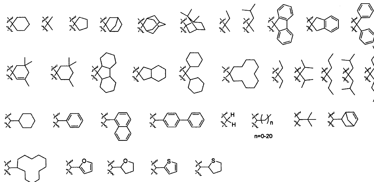
[Chem. 12]
