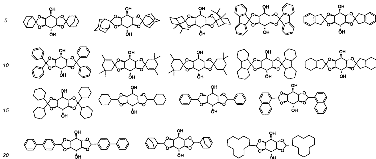
[Chem. 18]
