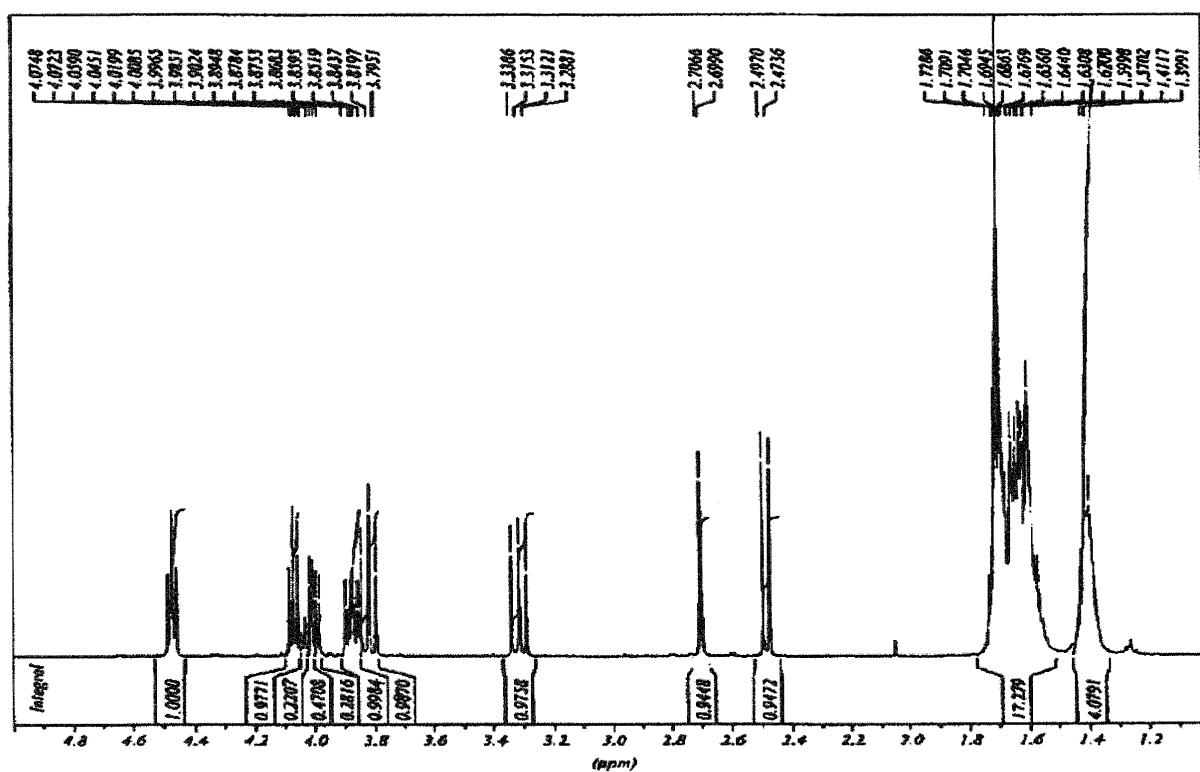
^1\text{H} -NMR SPECTRUM OF DCMI MONOMER
