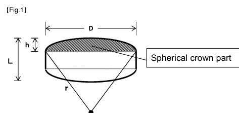
(A method for the calculation of the surface area of a tablet having the radius of curvature : r)
