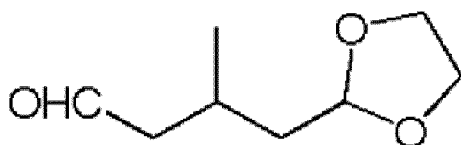
Compound B
