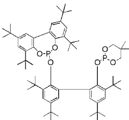
Bisphosphite A
