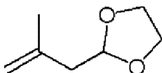
Compound A
