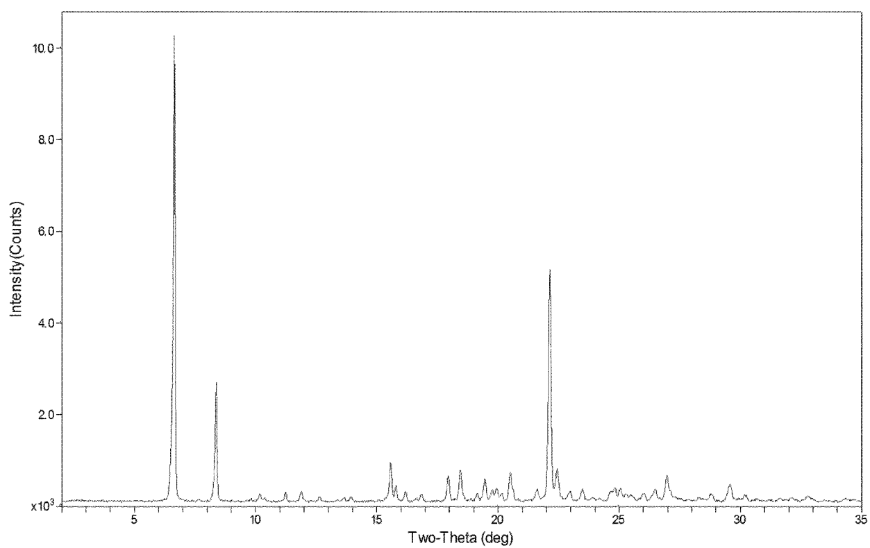
Figure 2-M: PXRD Pattern of Monohydrochloride Salt, Crystalline Form II
