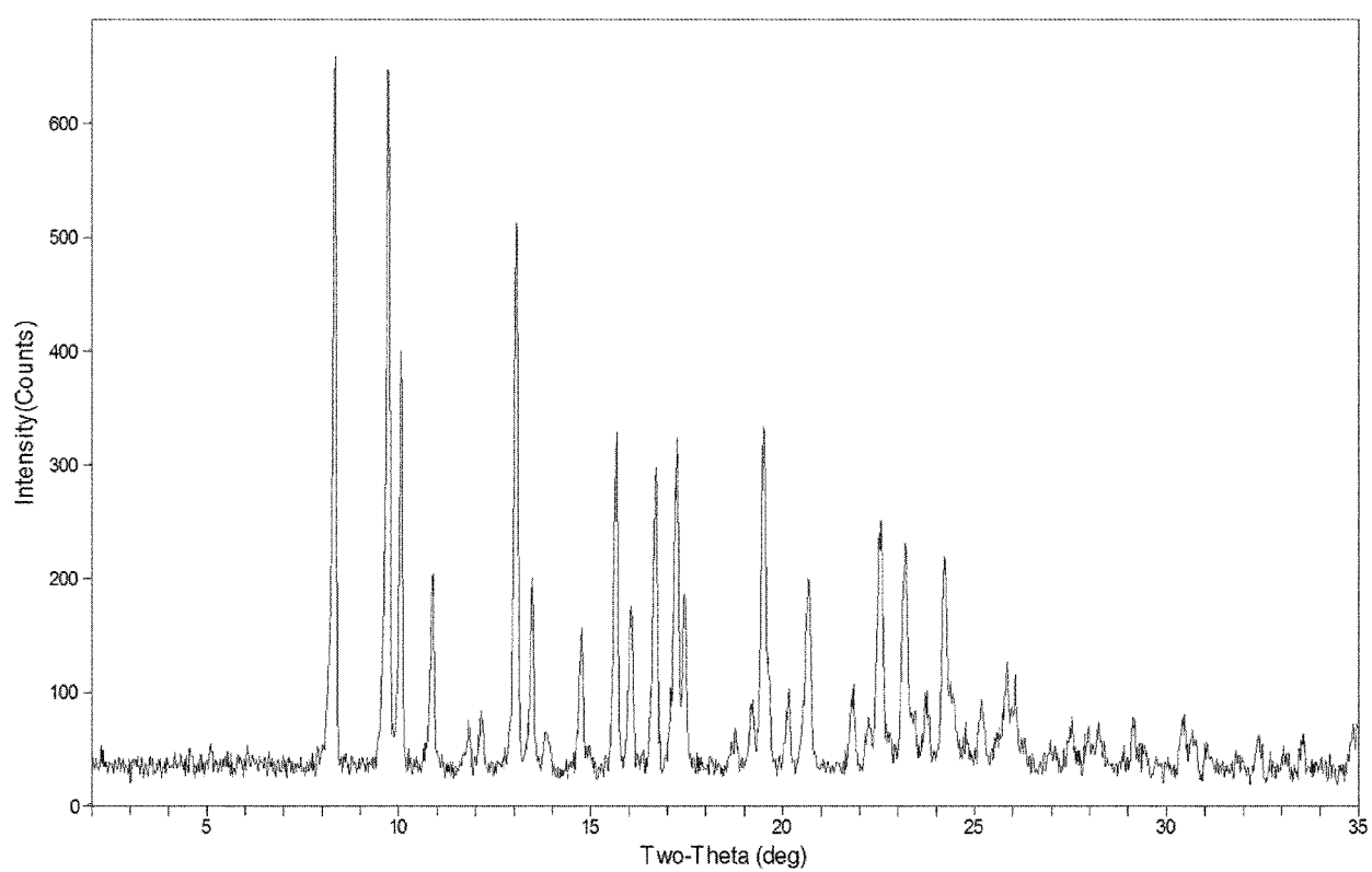
Figure 2-L: PXRD Pattern of Monohydrochloride Salt, Crystalline Form I
