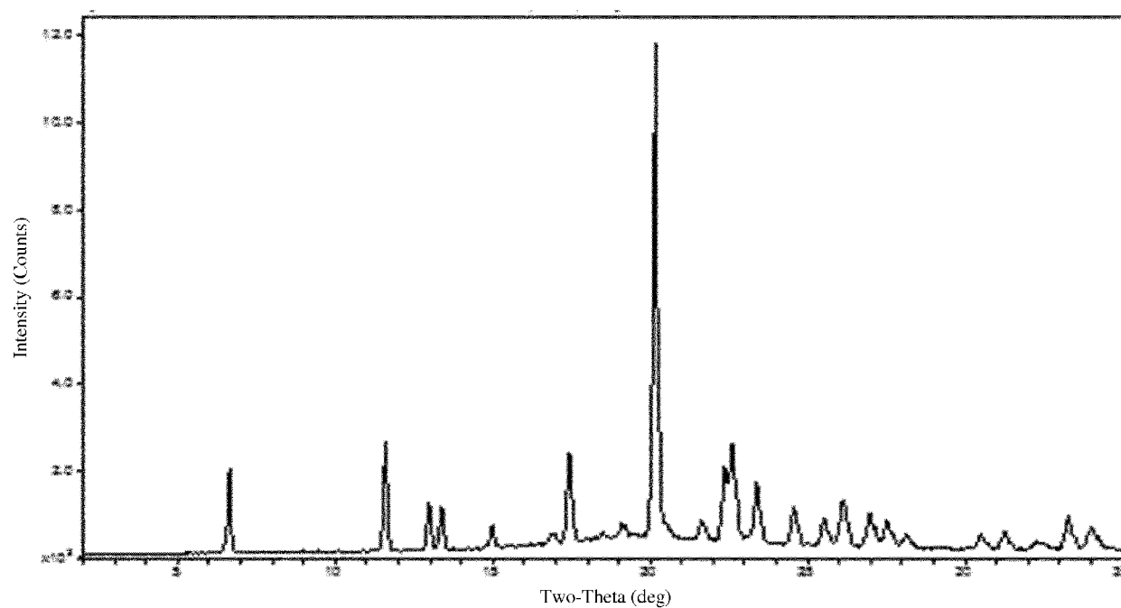
Figure 2-E: PXRD Pattern of S-Mandelate Salt (1:1 Stoichiometry), Crystallized From Pyridine
