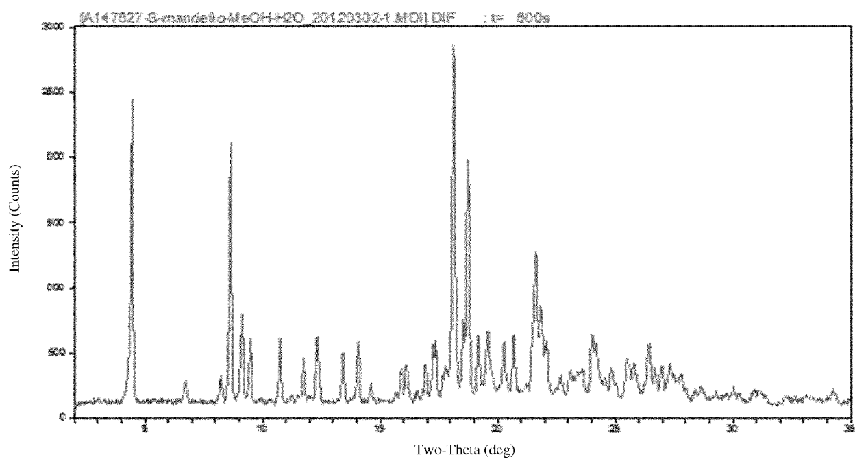
Figure 2-F: PXRD Pattern of S-Mandelate Salt (2:1 Stoichiometry), Hydrate
