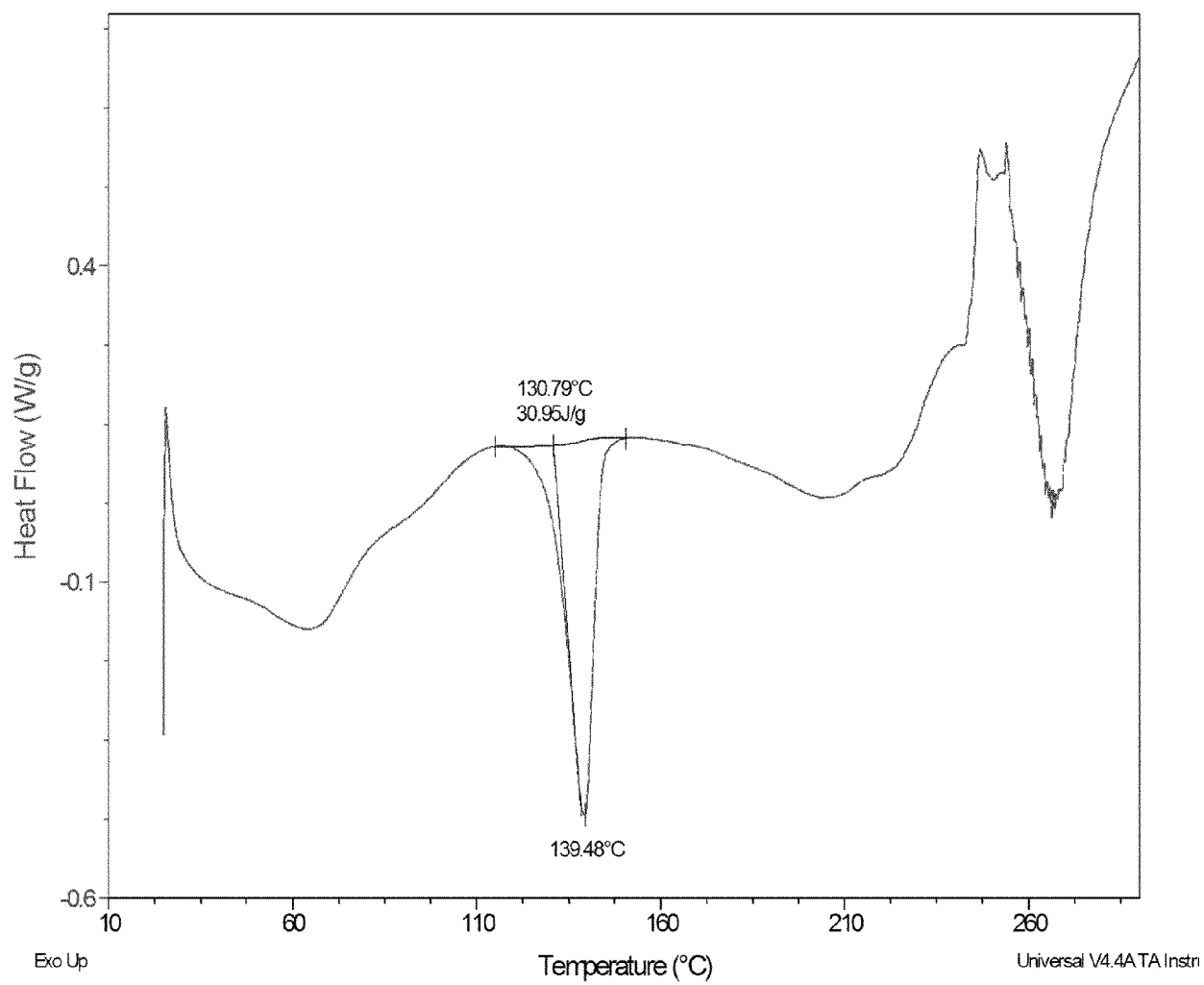
Figure 7-A: Differential Scanning Calorimetry Curve Hemi-Sulfate Salt (1:1 Stoichiometry), Monohydrate
