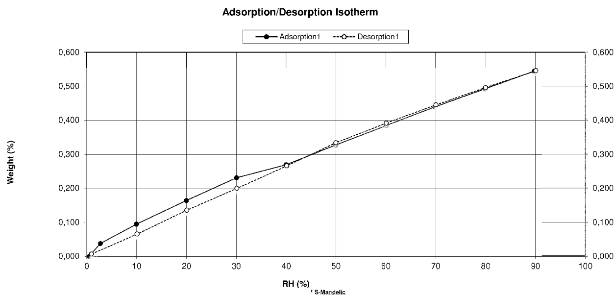
Figure 6-B: Moisture Sorption Isotherm S-Mandelate Salt (1:1 Stoichiometry), Anhydrate
