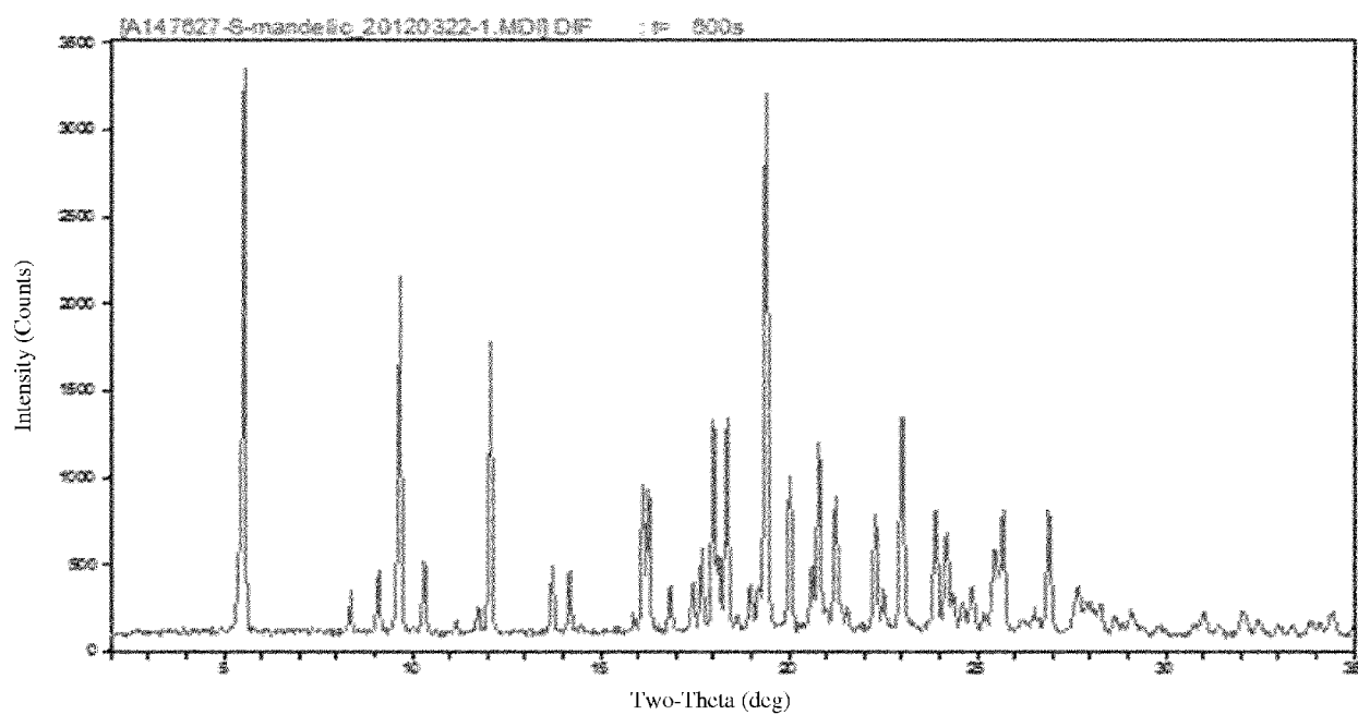
Figure 2-B: PXRD Pattern of S-Mandelate Salt (1:1 Stoichiometry), Anhydrate
