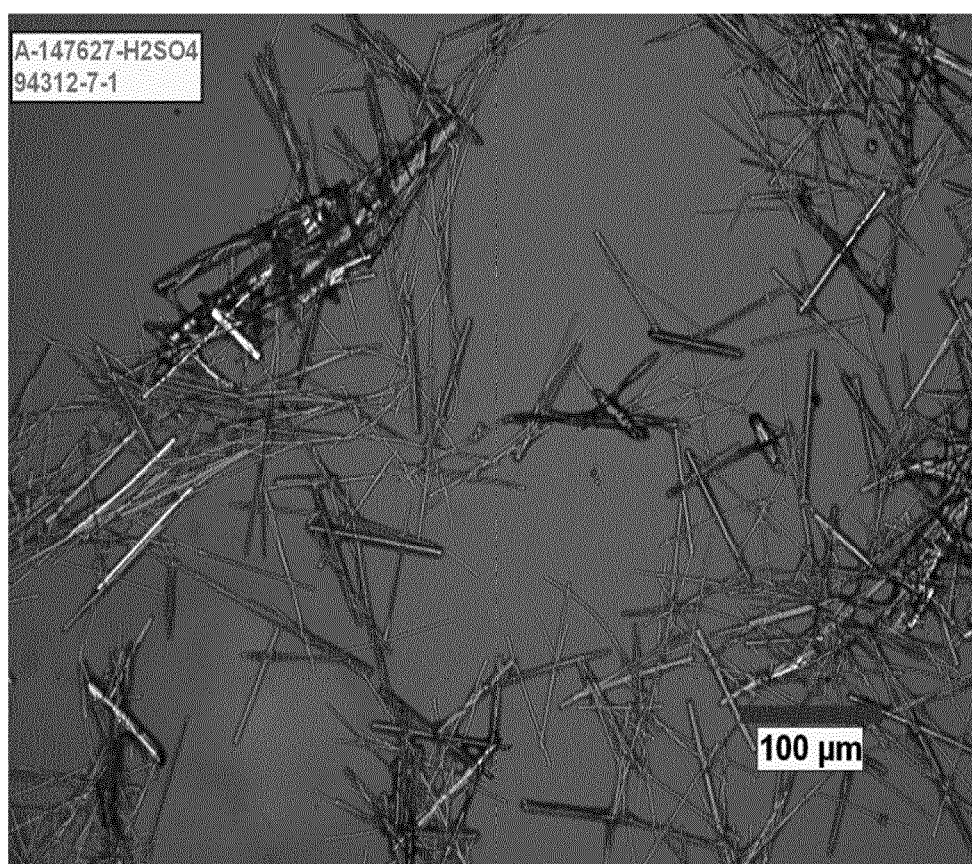
Figure 1-A: Microscopic Image of Hemi-Sulfate Salt (1:1 Stoichiometry), Monohydrate
