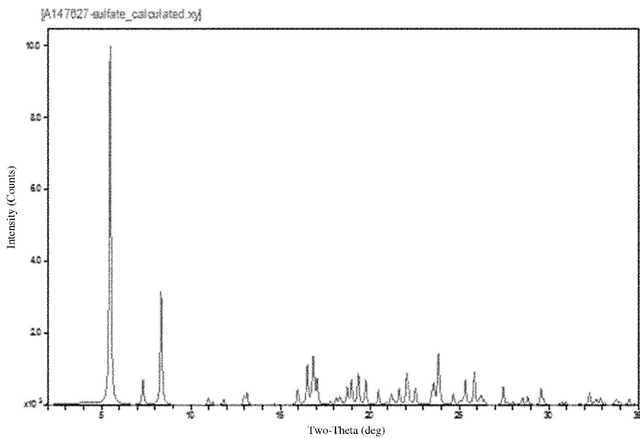
Figure 2-A: PXRD Pattern of Hemi-Sulfate Salt (1:1 Stoichiometry), Monohydrate
