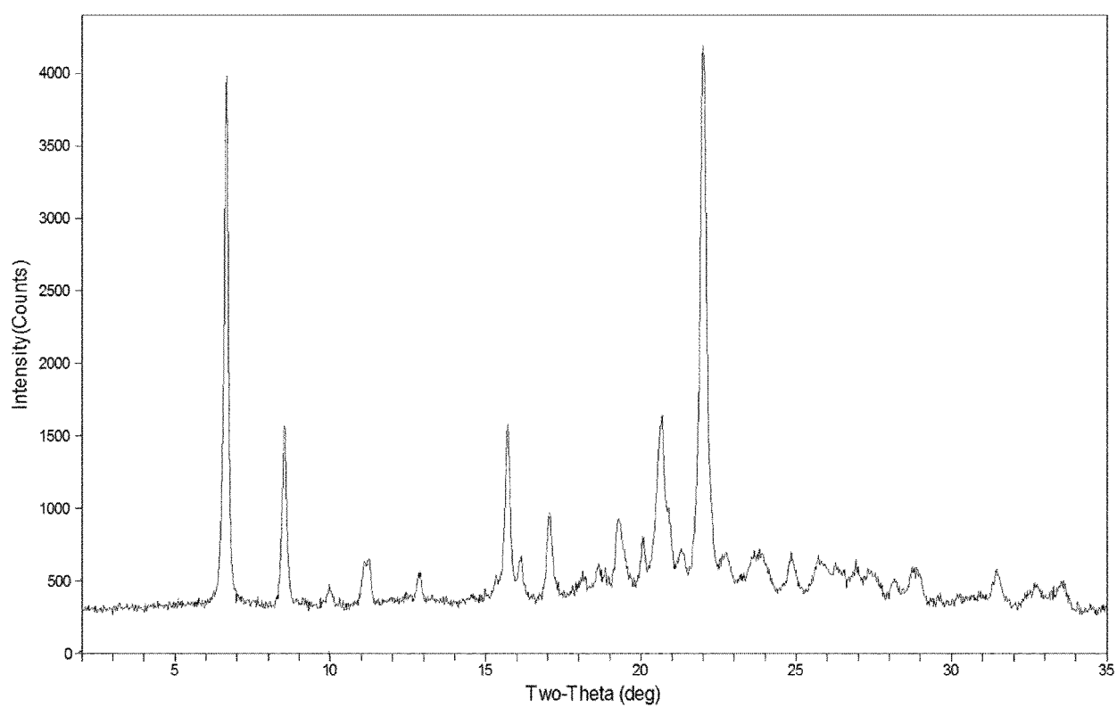
Figure 2-N: PXRD Pattern of Monohydrochloride Salt, Crystalline Form III
