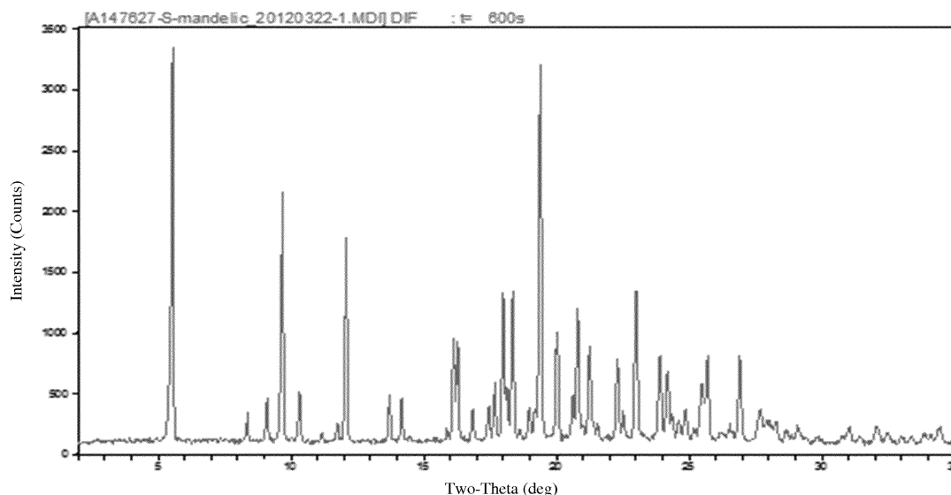
Figure 2-B: PXRD Pattern of S-Mandelate Salt (1:1 Stoichiometry), Anhydrate
