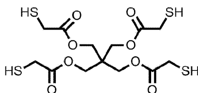
Chemical formula 1-1-1
