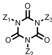
Chemical Formula 2-1
