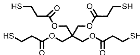
Chemical Formula 1-2-3
