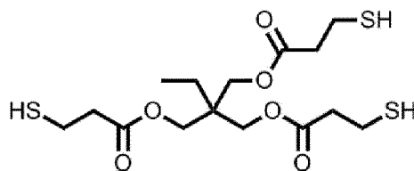
Chemical Formula 1-2-2
