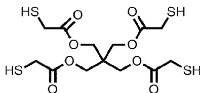
Chemical Formula 1-1-1
