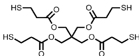
Chemical Formula 1-2-2
