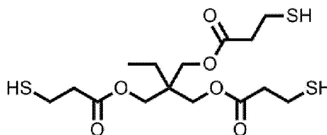
Chemical Formula 1-2-2
