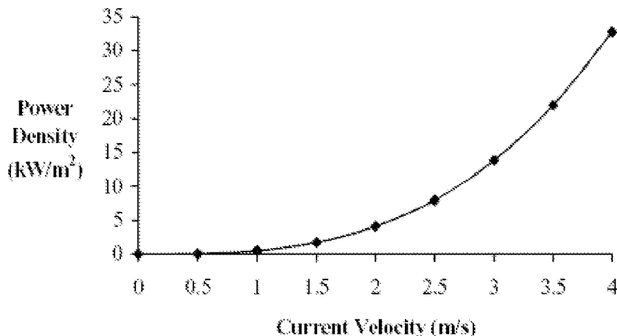
Figure 1-6: Incident Power Density as a Function of Current Speed
