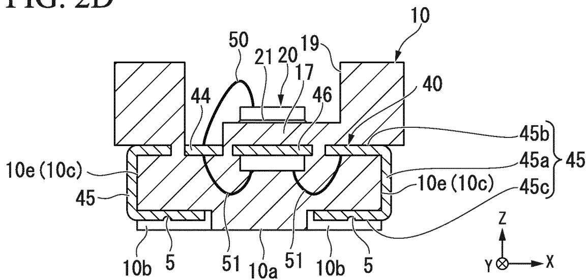
FIG. 2D
