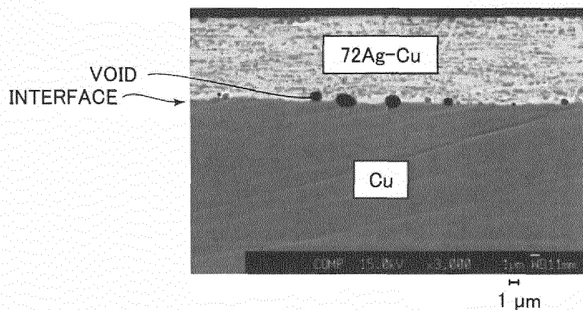
FIG.23 SECTIONAL PHOTOGRAPH ACCORDING TO COMPARATIVE EXAMPLE 12 (72Ag-Cu/Ni)
