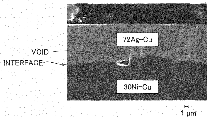
FIG.24 SECTIONAL PHOTOGRAPH ACCORDING TO COMPARATIVE EXAMPLE 13 (72Ag-Cu/30Ni-Cu)
