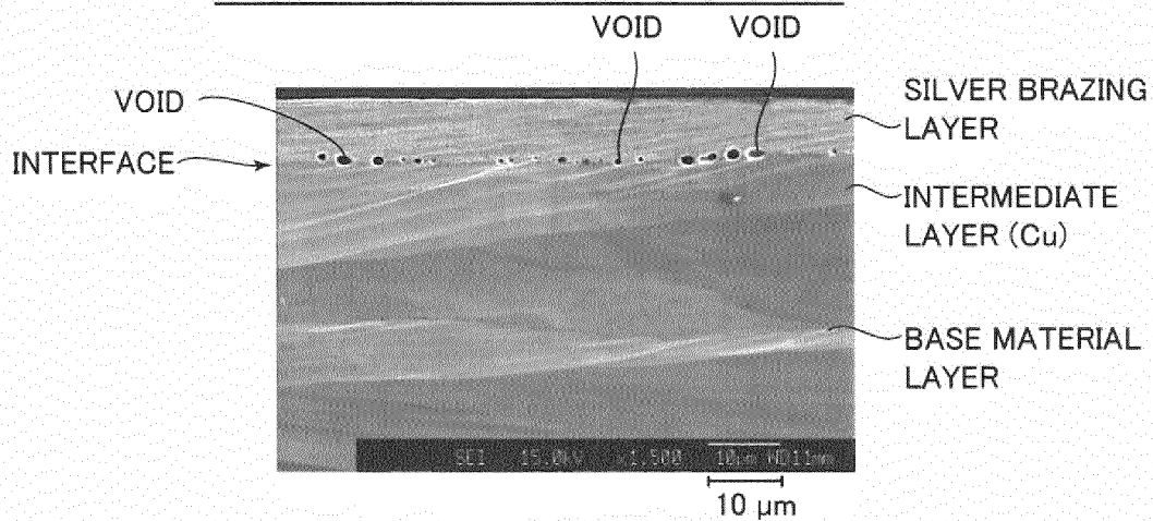
SECTIONAL PHOTOGRAPH ACCORDING TO COMPARATIVE EXAMPLE 1
