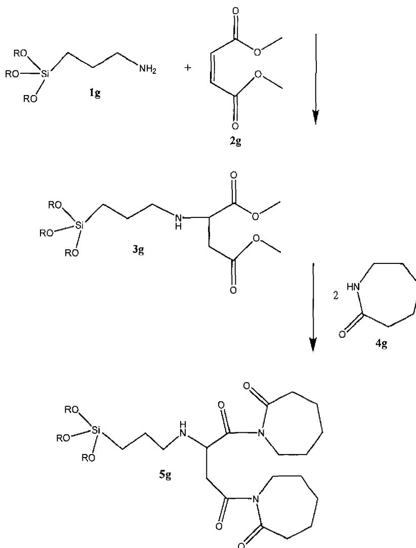
Exemplary Reaction Scheme (G)
