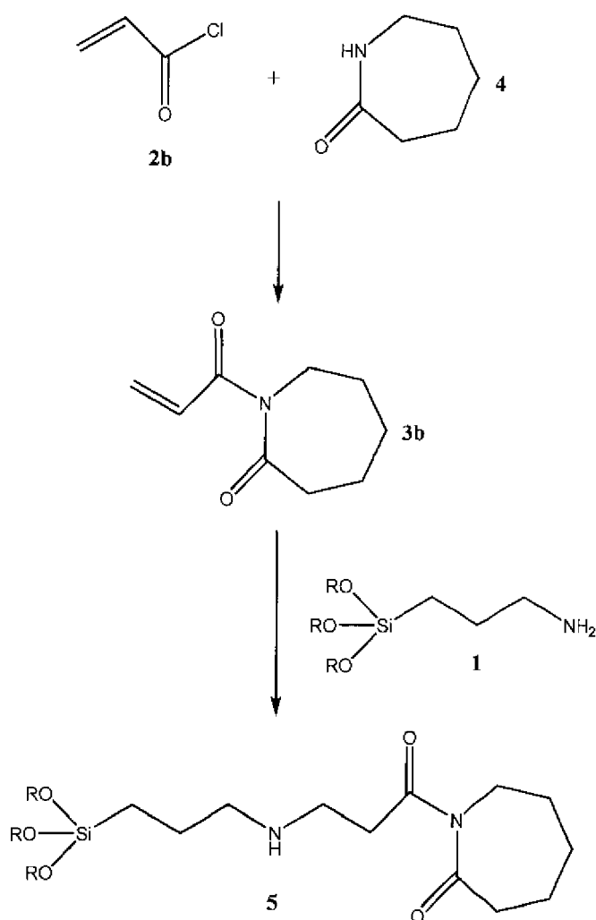
Exemplary Reaction Scheme (B)
