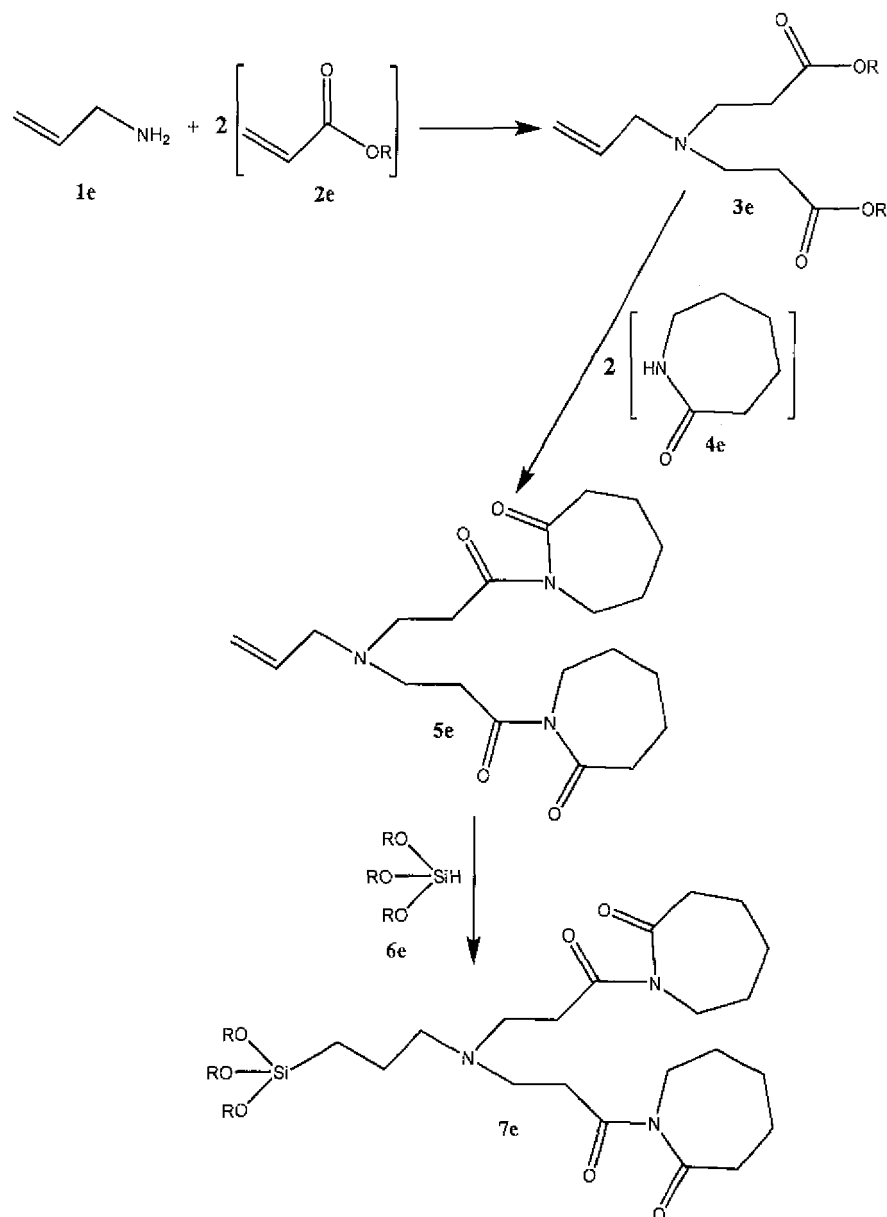
Exemplary Reaction Scheme (E)
