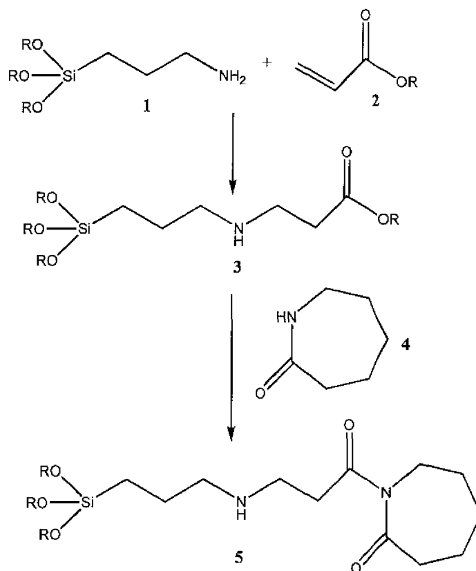
Exemplary Reaction Scheme (A)
