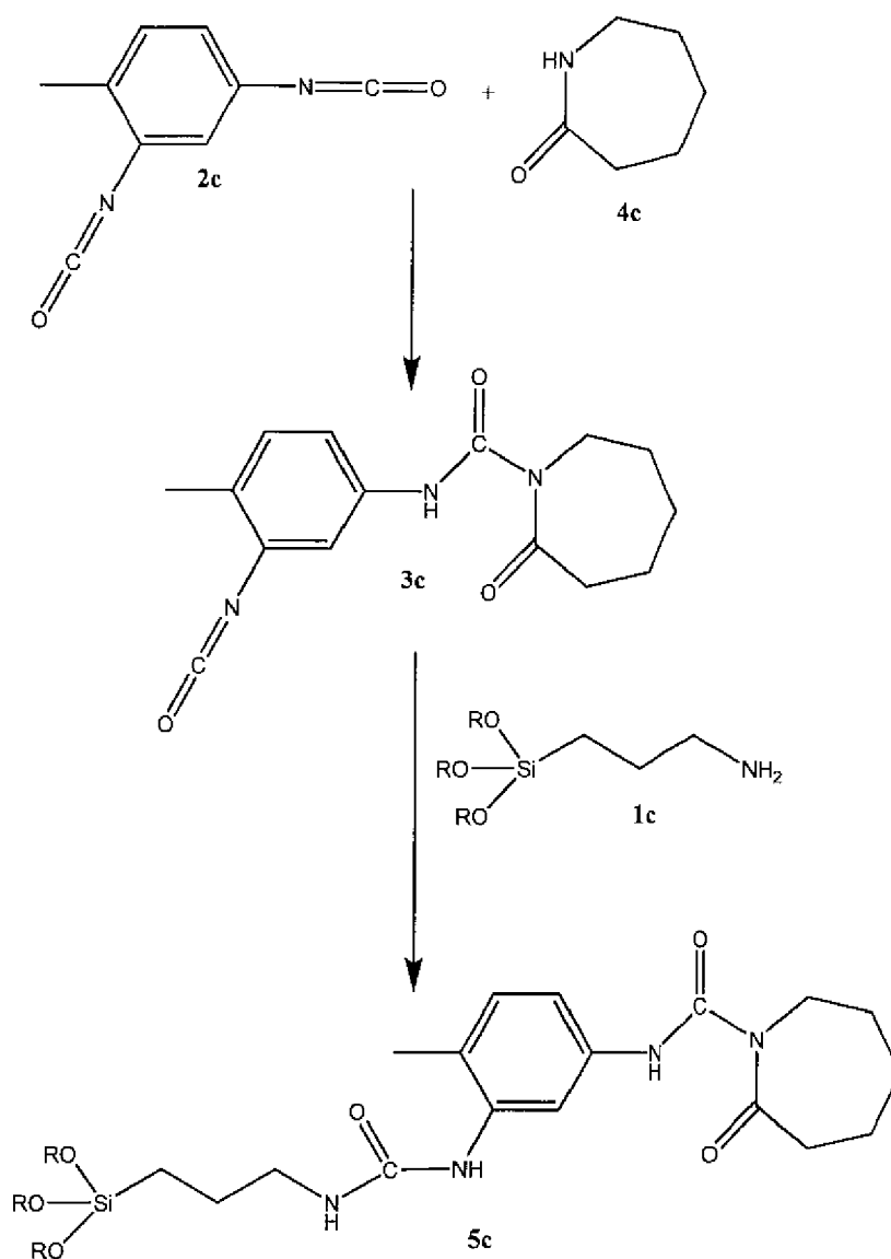
Exemplary Reaction Scheme (C)
