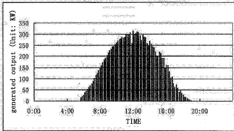
photovoltaic power output during a sunny weather
