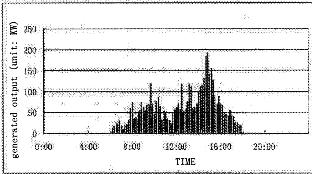
photovoltaic power output during a cloudy weather
