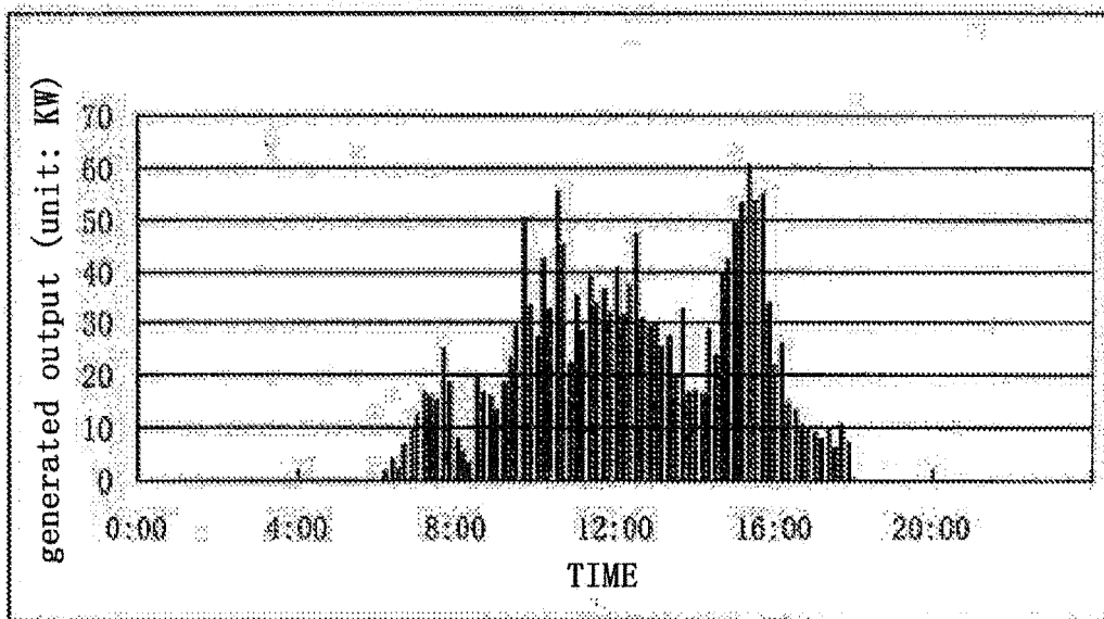
photovoltaic power output during a rainy weather
